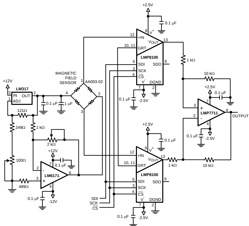
Figure 19. Bridge Amplifier
