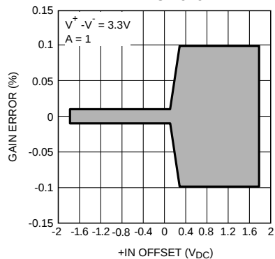
Small Signal Gain Error
