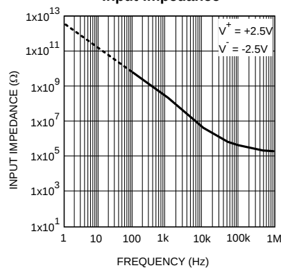
Input Impedance
