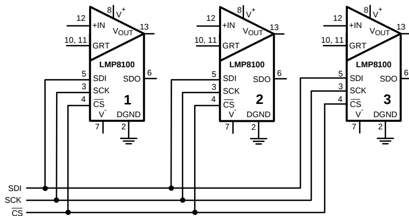
Figure 16. Star Configuration
