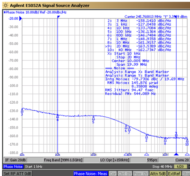
Figure 3-1. LMK04828B DCLKout2 Phase Noise VCO_MUX = 0 (VCO0) VCO0 = 2457.6 MHz DCLKout2_MUX = 0 (Divider) DCLKout2_DIV = 10 DCLKout2 Frequency = 245.76 MHz LVPECL20 /w 240 Ω emitter resistors CLKout2_3_IDL=1 CLKout2_3_ODL=0 Balun ADT2-1T+
