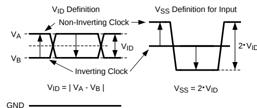
Figure 4-1. Two Different Definitions for Differential Input Signals
