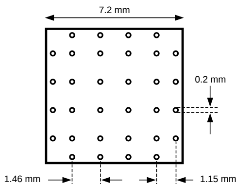
Figure 9-20. Recommended Land and Via Pattern
