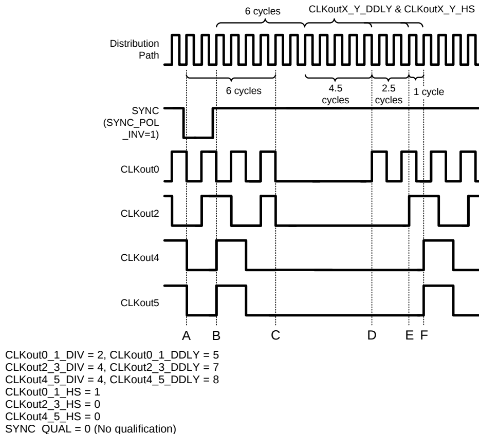
Figure 7-3. Clock Output synchronization using the SYNC pin (Active Low)
