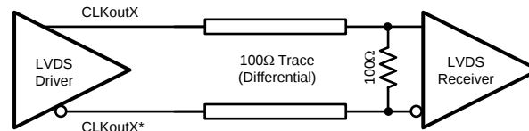
Figure 9-11. Differential LVDS Operation, DC Coupling, No Biasing of the Receiver
