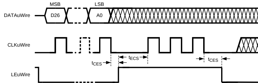
Figure 3-3. MICROWIRE Timing Diagram: Extra CLKuWire Pulses for R0 to R5 with LEOuWire Asserted
