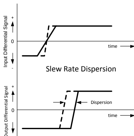
Figure 8. Slew Rate Dispersion
