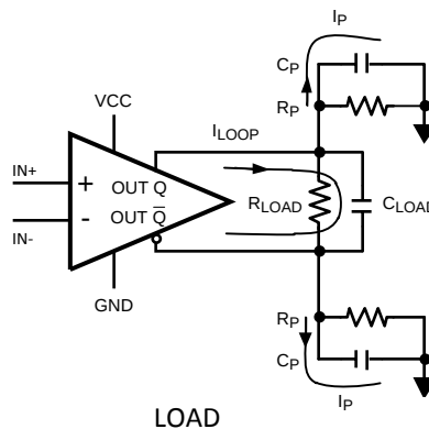
Figure 15. Load
