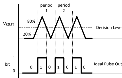
Figure 16. Bitrate
