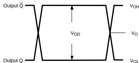
Figure 13. LVDS Output Signals
