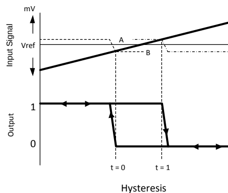
Figure 12. Hysteresis
