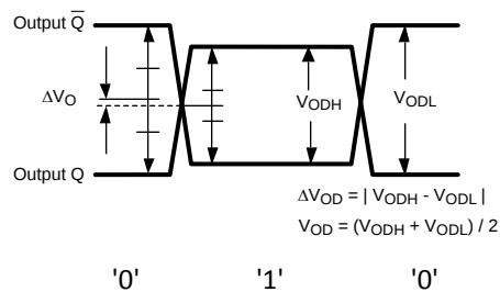
Figure 14. LVDS Output Signals with Different Amplitude
