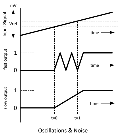
Figure 10. Oscillations & Noise
