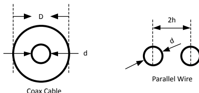
Figure 17. Cable Configuration
