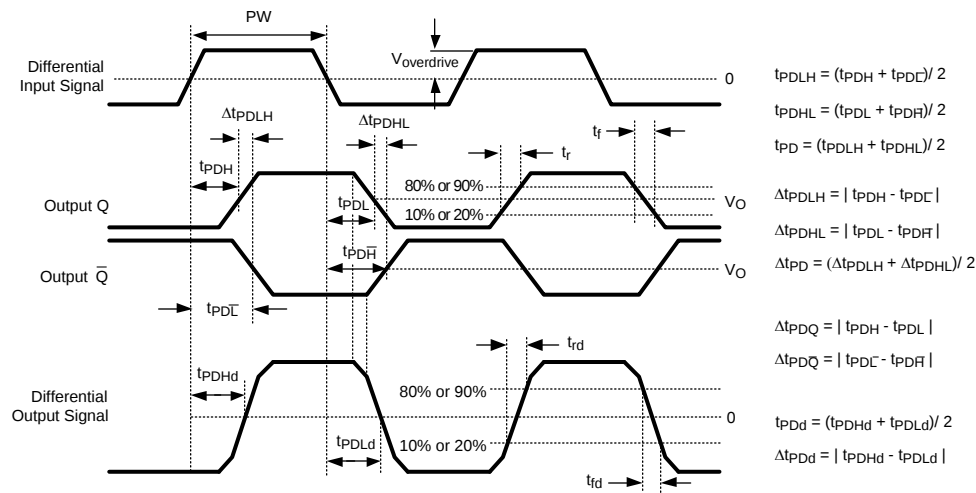
Figure 4. Propagation Delay Definition
