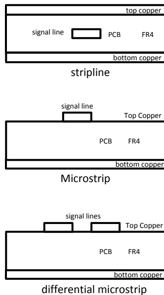
Figure 18. PCB Transmission Lines
