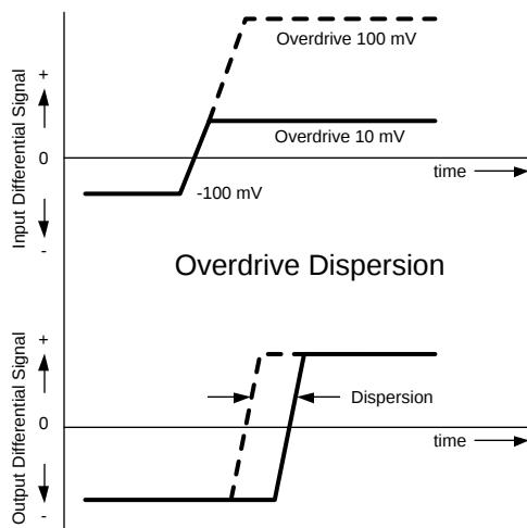
Figure 7. Overdrive Dispersion
