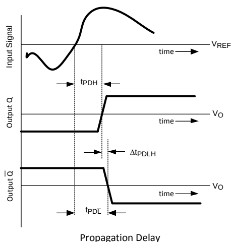
Figure 6. Propagation Delay
