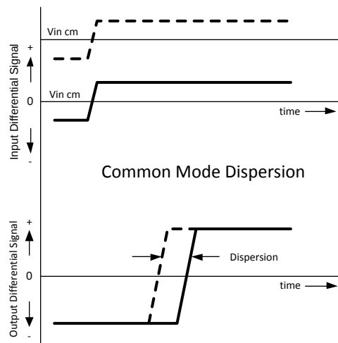
Figure 9. Common Mode Dispersion
