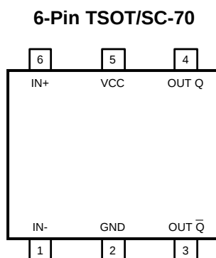
Figure 1. Top View
