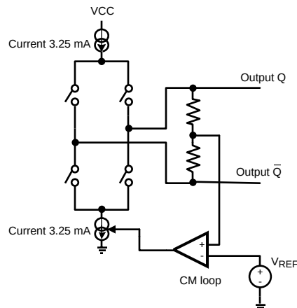
Equivalent Output Circuitry
