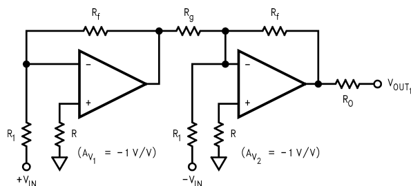
Figure 8. Differential Line Receiver
