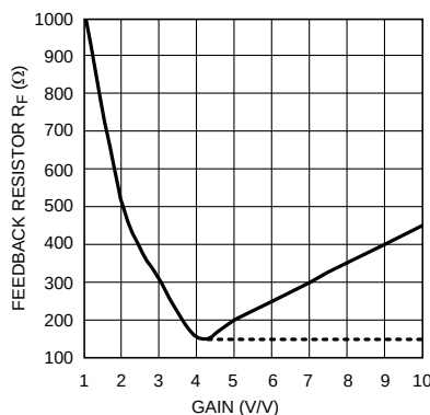
Figure 5. R_F vs. Non-Inverting Gain
