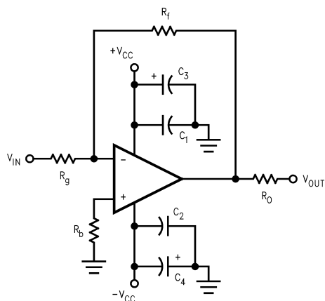
Figure 3. Inverting Configuration with Power Supply Bypassing
