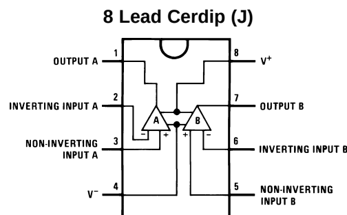
Figure 1. Top View
