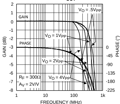
Frequency Response
