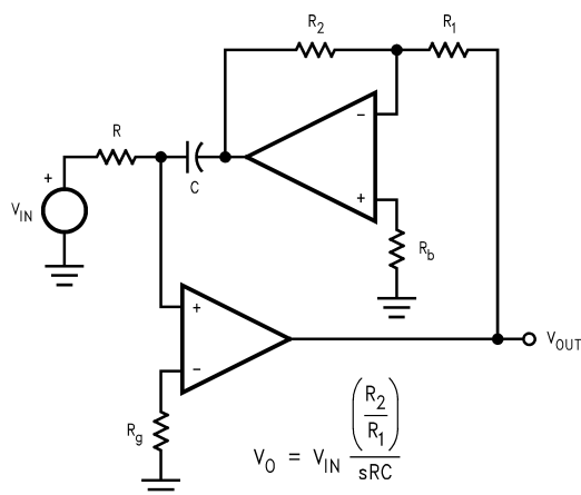
Figure 10. Current Feedback Integrator
