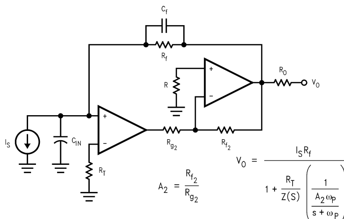
Figure 11. Low-Noise, Wide Bandwidth, Transimpedance Amp.
