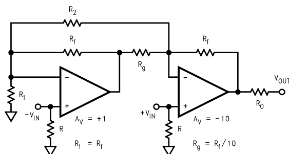
Figure 9. Differential Line Receiver with CMRR Adjustment
