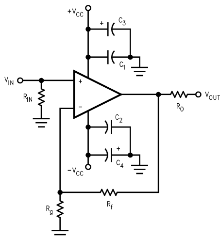
Figure 2. Non-Inverting Configuration with Power Supply Bypassing
