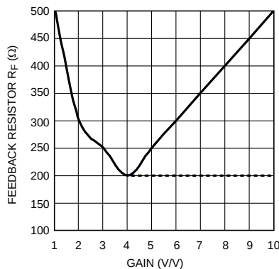
Figure 6. R_F vs. Inverting Gain
