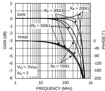
Figure 4. Frequency Response vs. R_F
