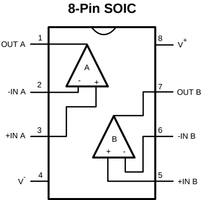
Figure 2. Top View
