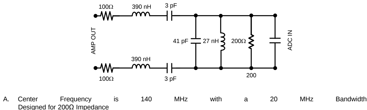
Figure 57. Bandpass Filter
