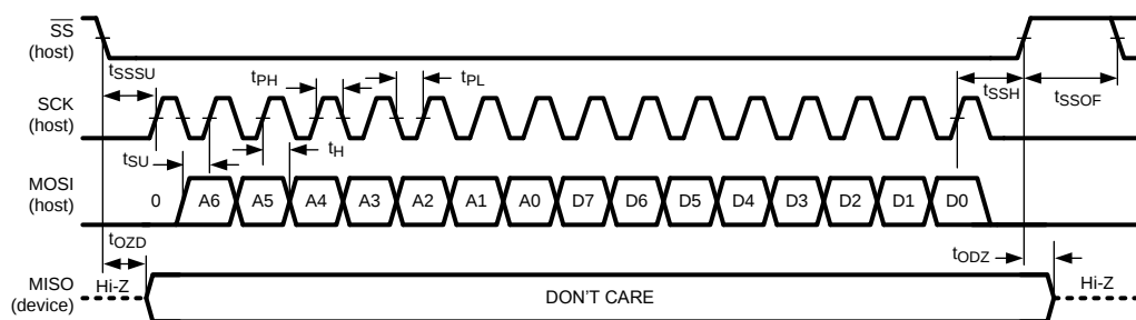
Figure 4. SPI Write
