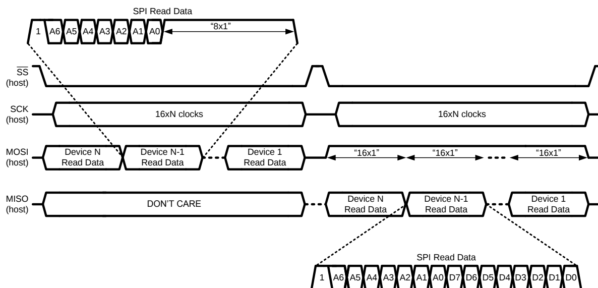
Figure 8. SPI Daisy-Chain Read
