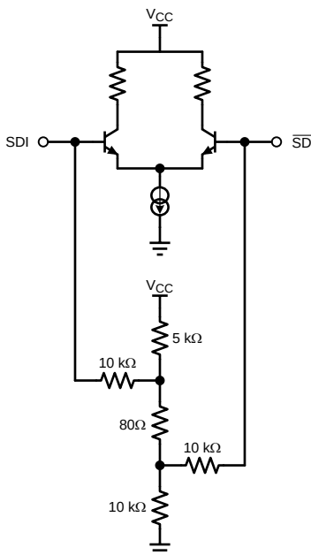
Figure 3. Differential Input Stage for \text{SDI} and \overline{\text{SDI}} .
