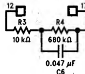
FIGURE 6. Enhanced Stereo Circuit
