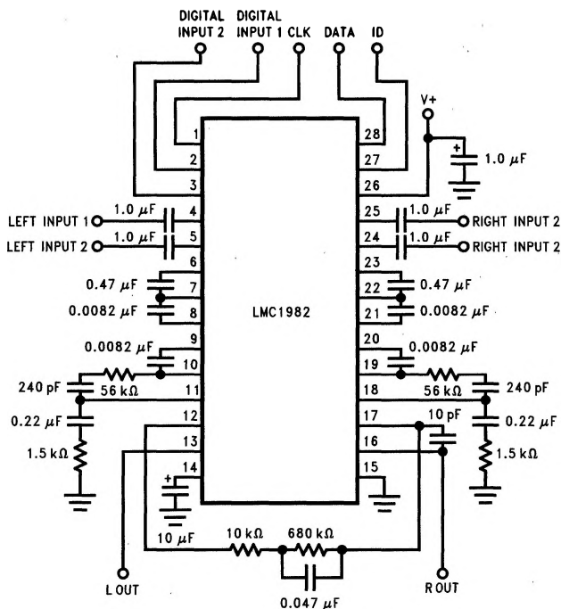
FIGURE 1. Typical Application
