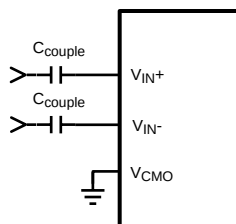
Figure 41. Differential Analog Input Connection
