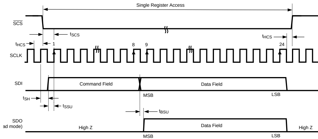
Figure 10. Serial Interface Timing
