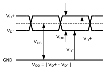
Figure 1. LVDS Output Signal Levels
