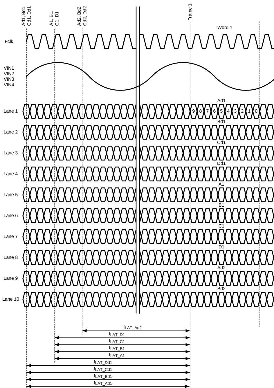
Figure 8. Latency - Quad ADC Mode
