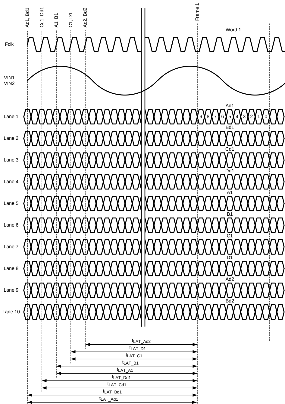
Figure 7. Latency - Dual ADC Mode
