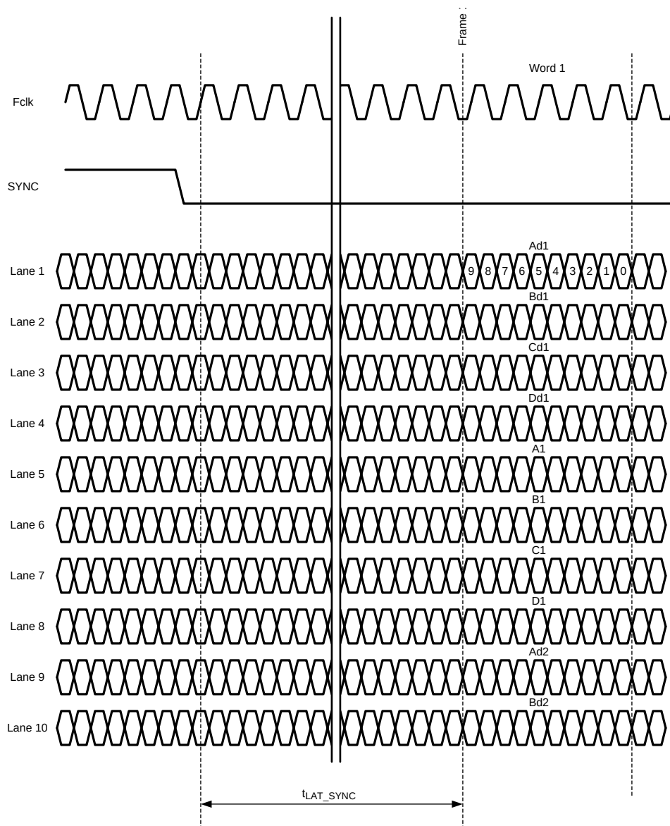
Figure 5. SYNC Timing - Falling Edge
