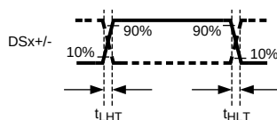
Figure 3. Output Data Timing
