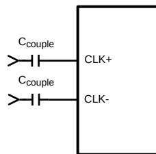
Figure 44. Differential Sample Clock Connection
