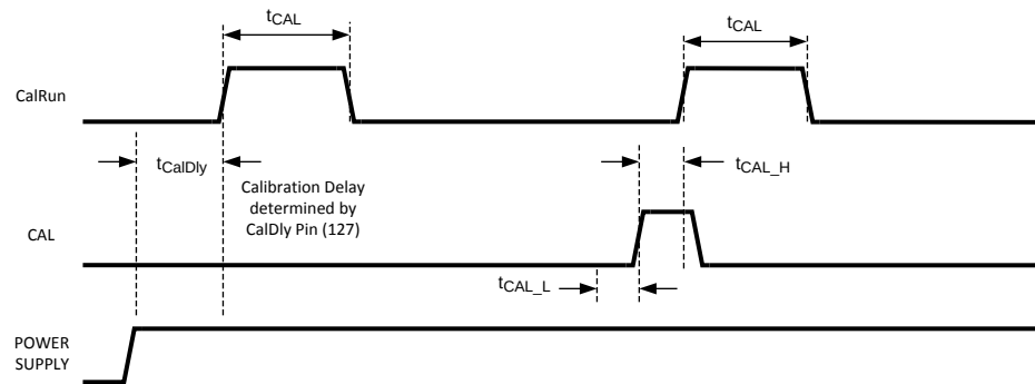
Figure 9. Calibration and On-Command Calibration Timing
