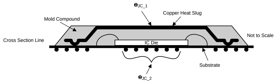
Figure 45. HSBGA Conceptual Drawing
