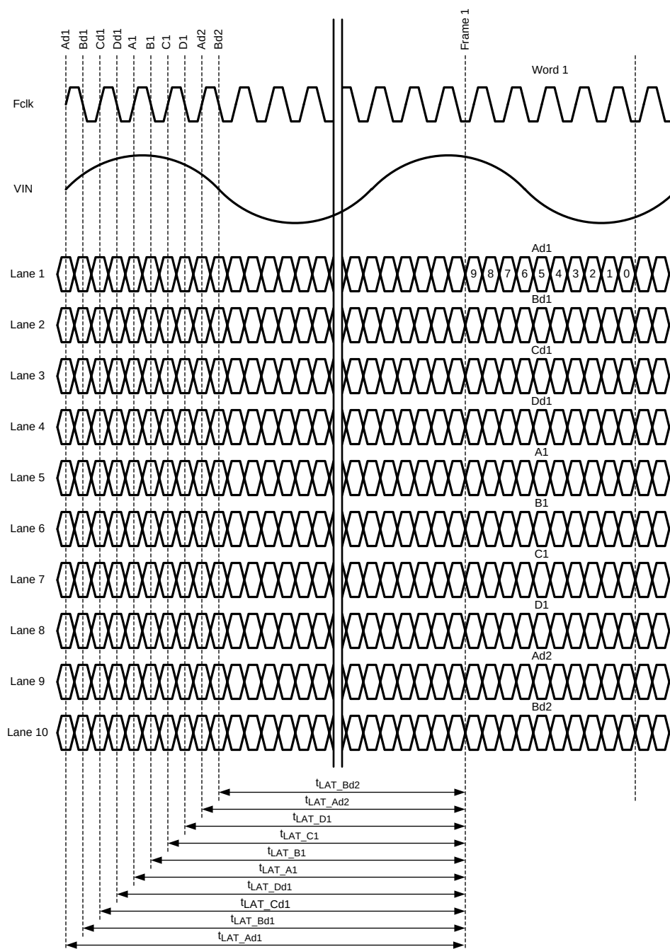
Figure 6. Latency - Single ADC Mode
