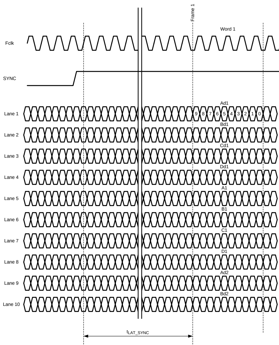
Figure 4. SYNC Timing - Rising Edge
