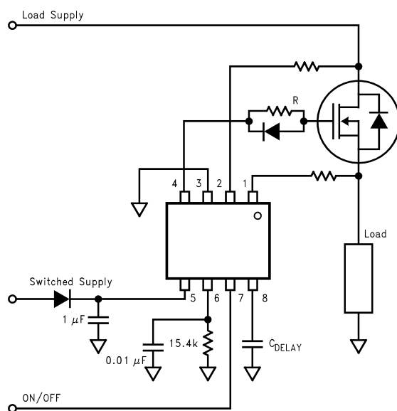
Figure 9. Increasing MOSFET Turn On Time
