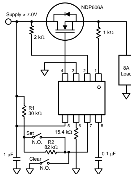
Figure 7. Electronic Circuit Breaker
