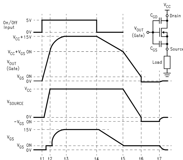
Figure 3. Turn ON and Turn OFF Waveforms
