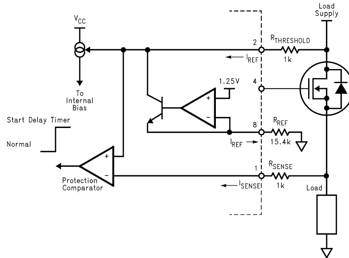
Figure 4. Protection Comparator Biasing
