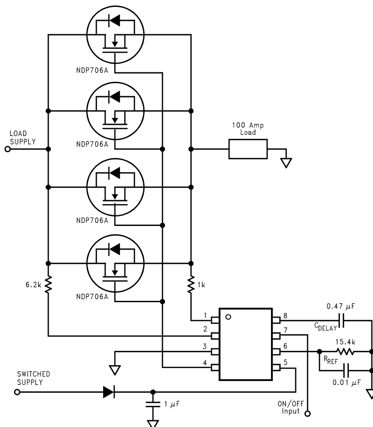
Figure 8. Driving Multiple MOSFETs
