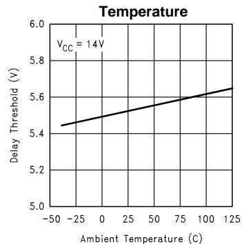
Delay Threshold vs Temperature
