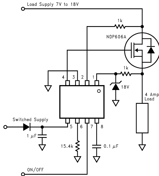
Figure 6. Adding Over-Voltage Protection
