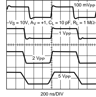
Step Response for Various Amplitudes
