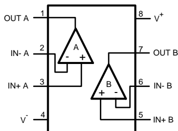
Figure 1. 8-Pin MSOP (Top View)
