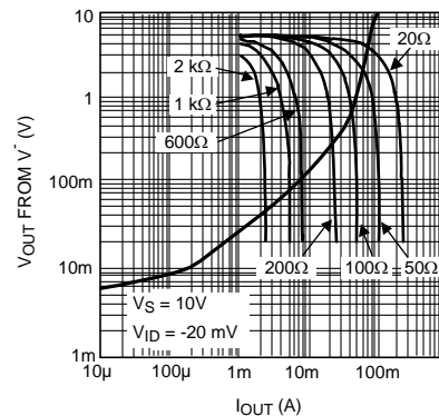
Figure 5. Steady State Output Sinking Characteristics with Load Lines
