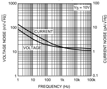
Input Referred Noise Density vs.
