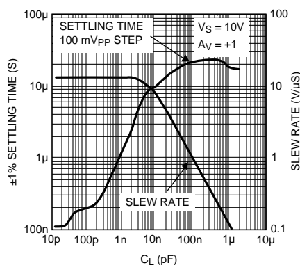
Figure 3. Settling Time and Slew Rate vs. Capacitive Load
