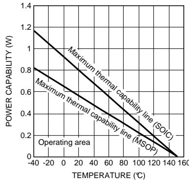
Figure 6. Power Capability vs. Temperature
