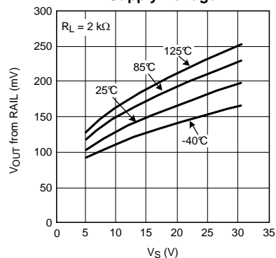
Negative Output Swing vs. Supply Voltage
