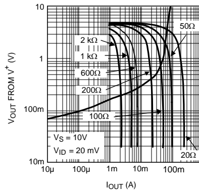
Figure 4. Steady State Output Sourcing Characteristics with Load Lines
