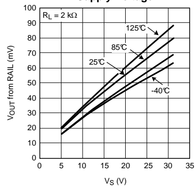
Negative Output Swing vs. Supply Voltage
