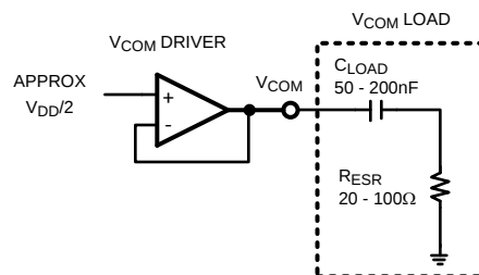
Figure 5. V_{COM} Driver with Simplified Load
