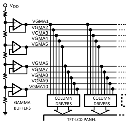
Figure 10. Basic Gamma Buffer Configuration
