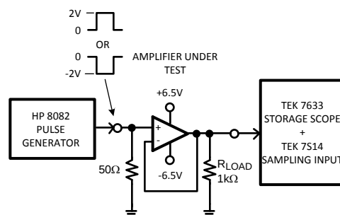
Figure 12. Gamma Buffer Settling Time Test Circuit
