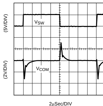
Figure 7. V_{SW} and V_{COM} Waveforms from V_{COM}
