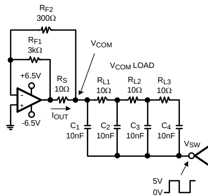
Figure 6. V_{COM} Driver Test Circuit
