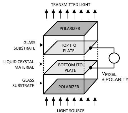
Figure 2. Individual LCD Pixel
