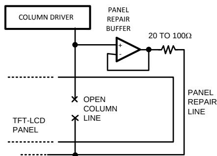
Figure 13. Panel Repair Buffer
