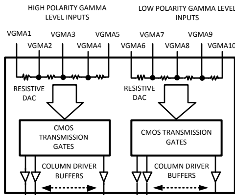
Figure 9. Simplified Schematic of Column Driver IC
