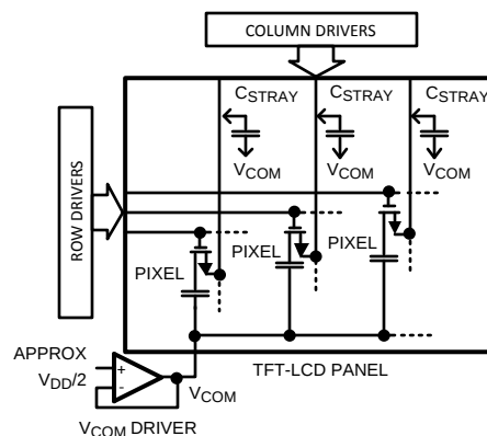
Figure 3. TFT Display
