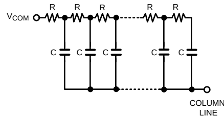
Figure 4. Model of Impedance between V_{COM} and Column Lines
