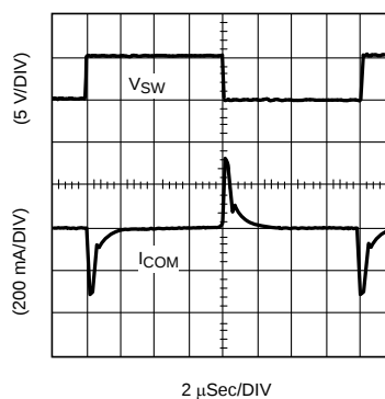
Figure 8. V_{SW} and I_{OUT} Waveforms from V_{COM} Test Circuit
