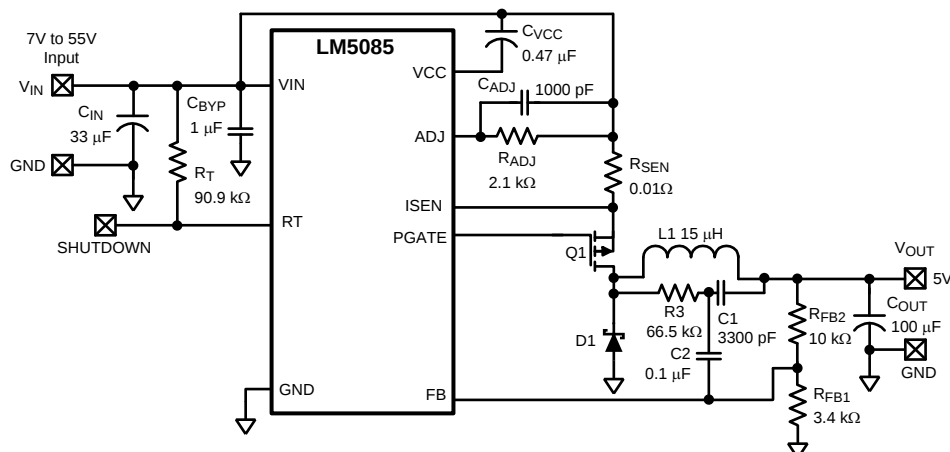
Figure 28. Example Circuit
