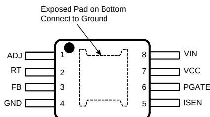
Figure 1. Top View 8-Lead MSOP-PowerPAD
