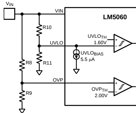
Figure 30. Programming the Thresholds with Resistors R8-R11
