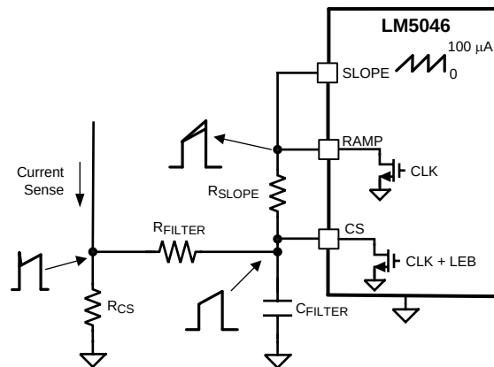
Figure 22. Current Mode Configuration
