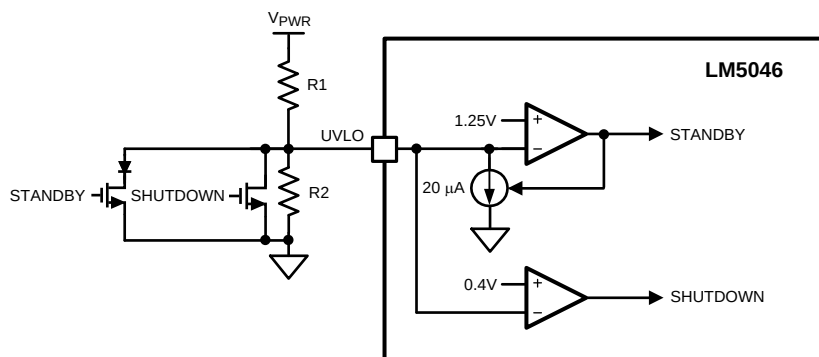
Figure 28. Remote Standby and Disable Control
