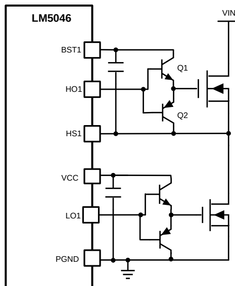
Figure 34. Bipolar Totem Pole Arrangement
