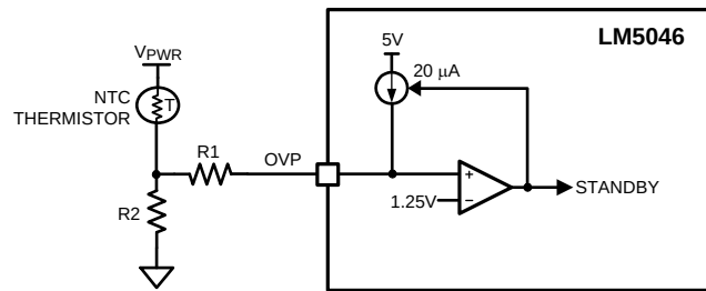
Figure 29. Remote Thermal Protection
