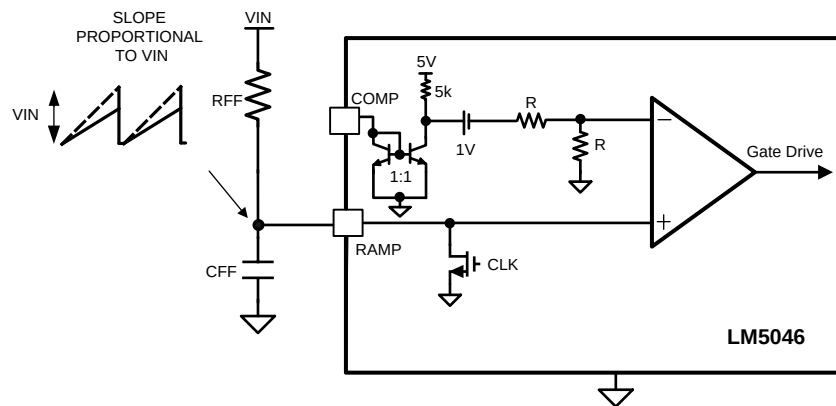
Figure 21. Feed-Forward Voltage Mode Configuration
