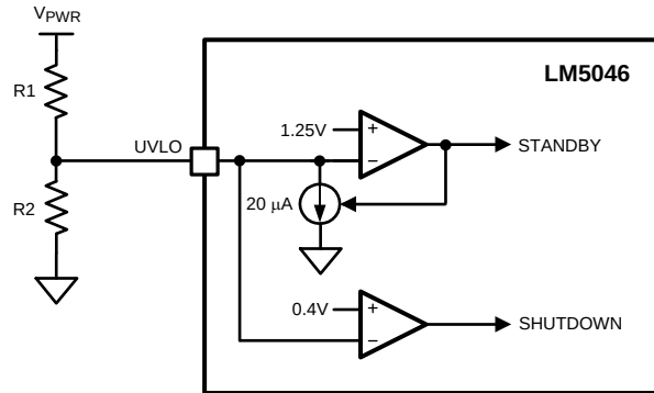
Figure 25. Basic UVLO Configuration
