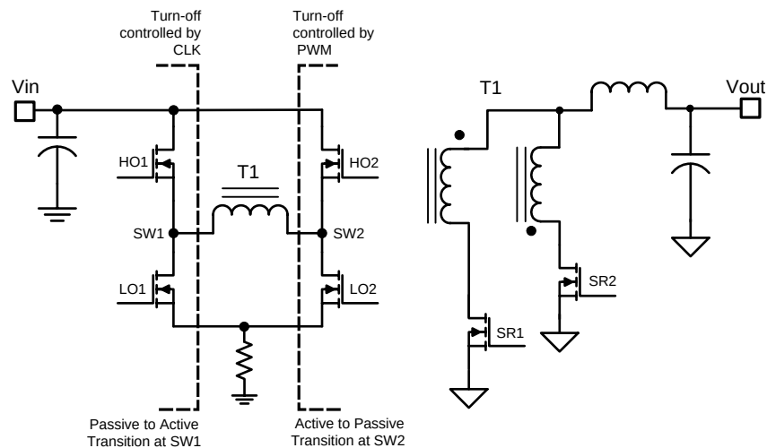
Figure 20. Simplified PSFB Topology Showing the Turn-Off Mechanism
