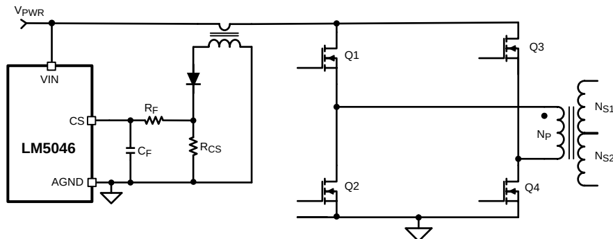
Figure 30. Transformer Current Sense
