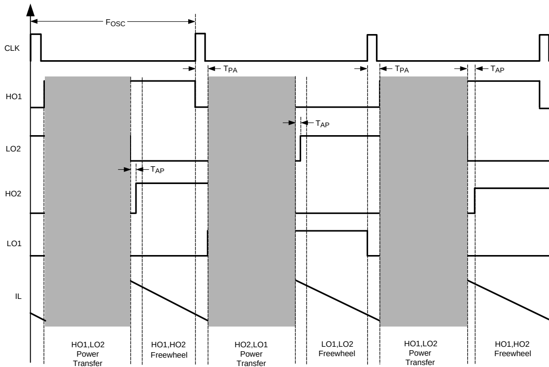
Figure 14. Timing Diagram Illustrating the Sequence of Gate-Driver Outputs in the PSFB Topology
