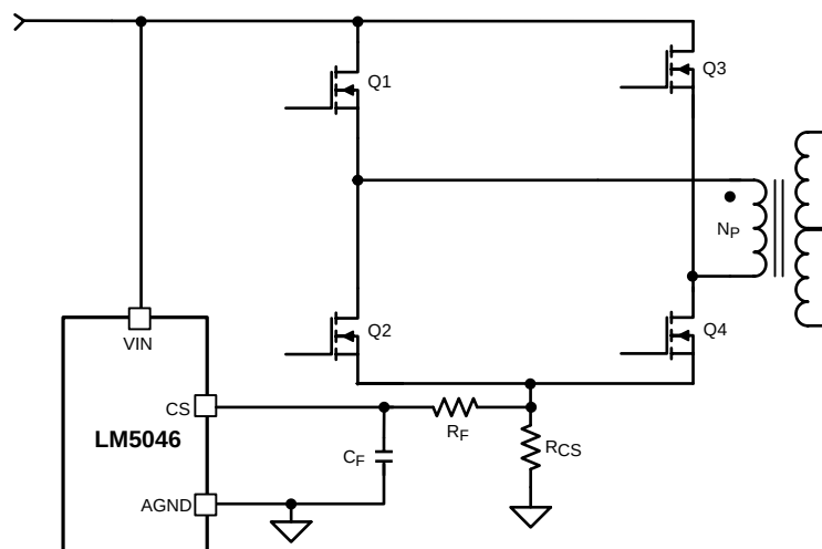
Figure 31. Resistor Current Sense
