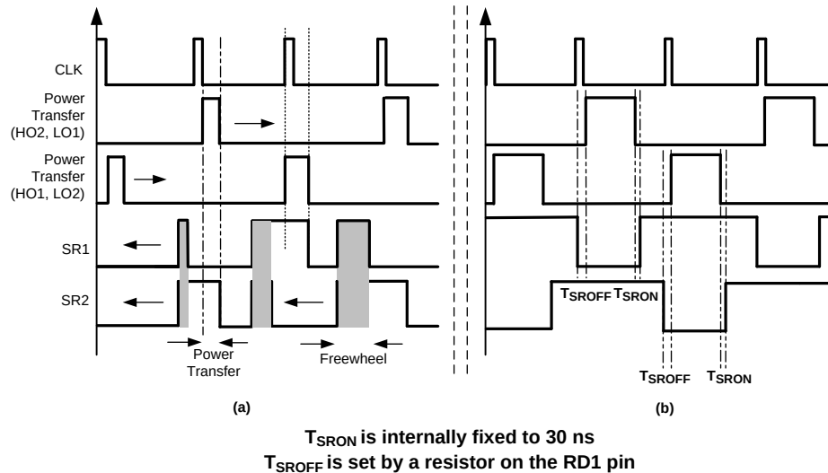
Figure 16. (a) Waveforms during Soft-Start (b) Waveforms after Soft-Start
