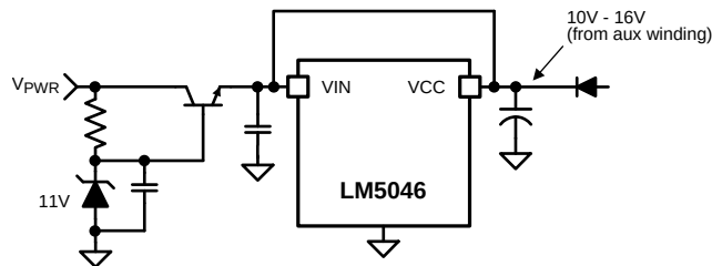
Figure 24. Start-Up Regulator for V_{PWR} > 100V
