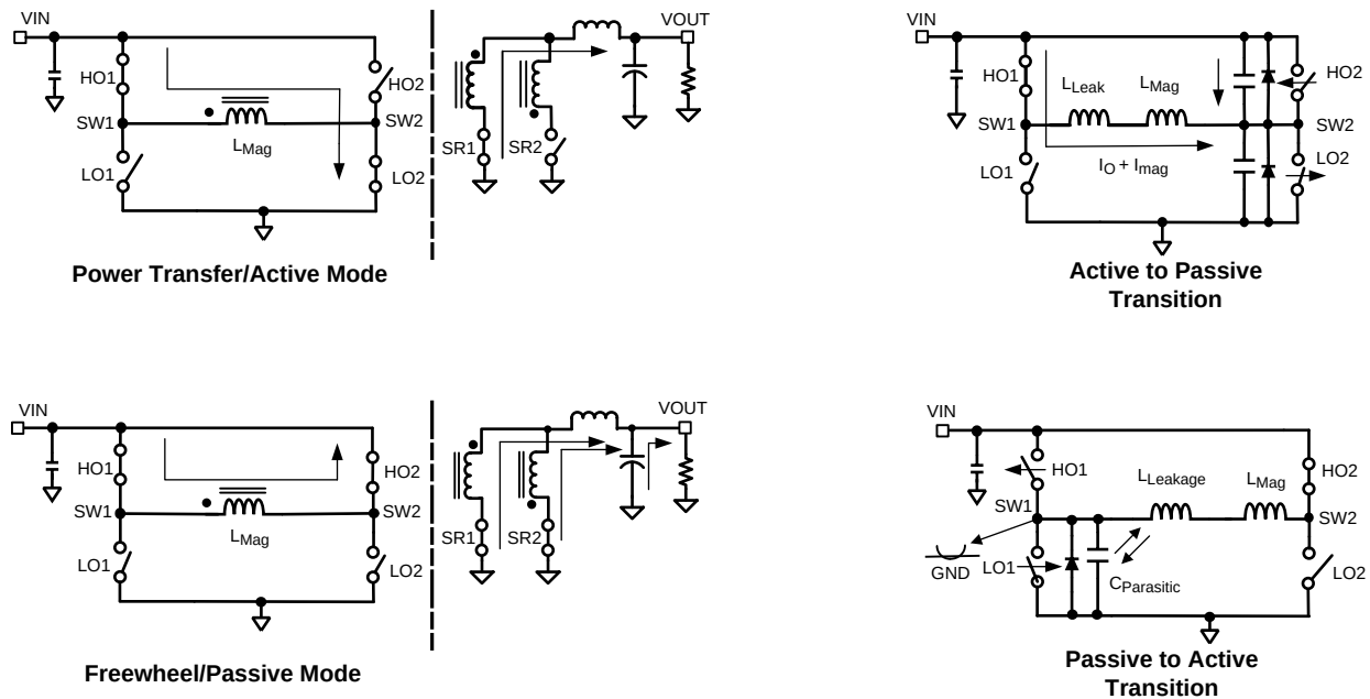
Figure 19. Operating States of the PSFB Topology
