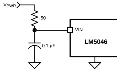
Figure 23. Input Transient Protection
