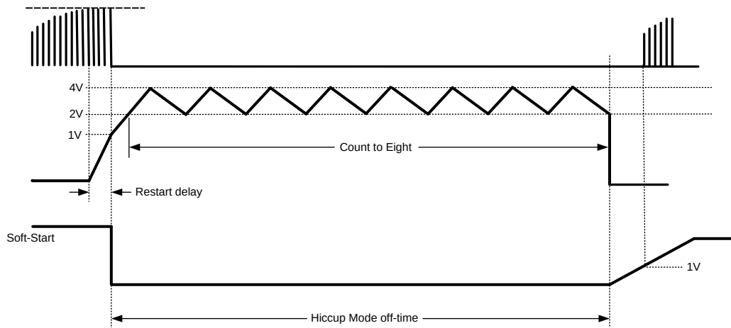
Figure 32. Hiccup Mode Delay and Soft-Start Timing Diagram
