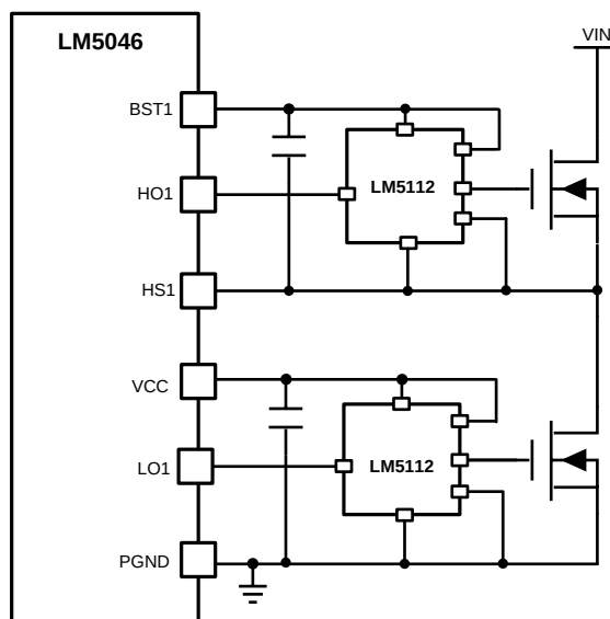
Figure 35. Using a Low Side Gate Driver to Augment Gate Drive Strength
