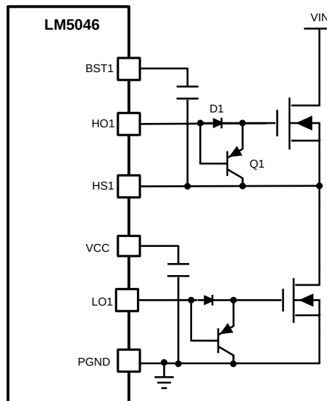
Figure 33. Circuit to Speed-up the Turn-off Process
