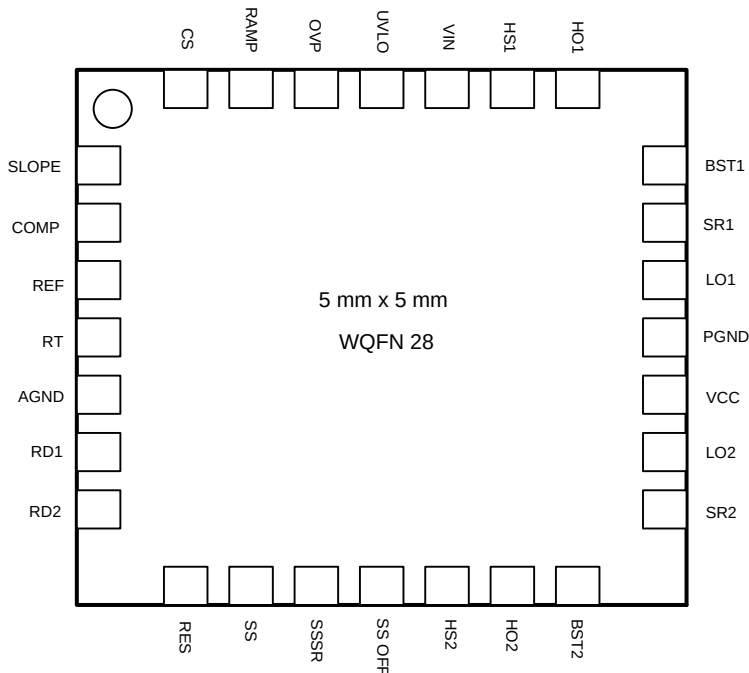
Figure 2. WQFN-28 Package Top View
