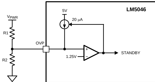
Figure 26. Basic OVP Configuration
