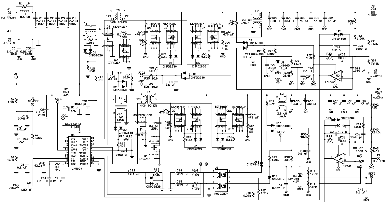
Figure 40. Dual Interleaved Regulator
