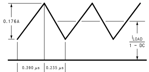
Figure 3. 10µH Inductor Current 5V - 12V Boost (LM4960)
