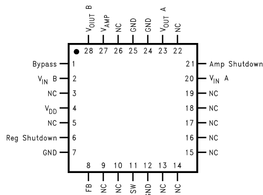
Figure 1. LM4960SQ (Top View)
