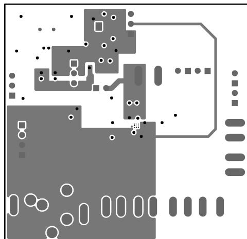
Figure 31. Layer 3
