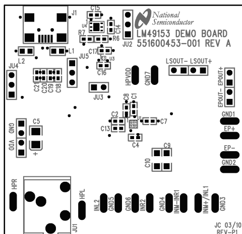
Figure 29. Top Silkscreen
