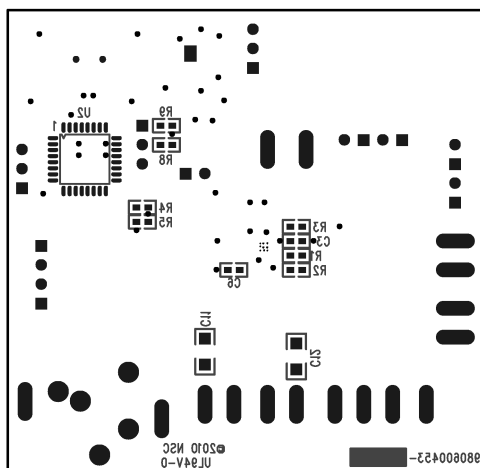
Figure 33. Bottom Silkscreen
