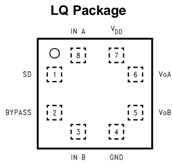
Figure 2. Top View Order Number LM4915LQ See NS Package Number LQB08A
