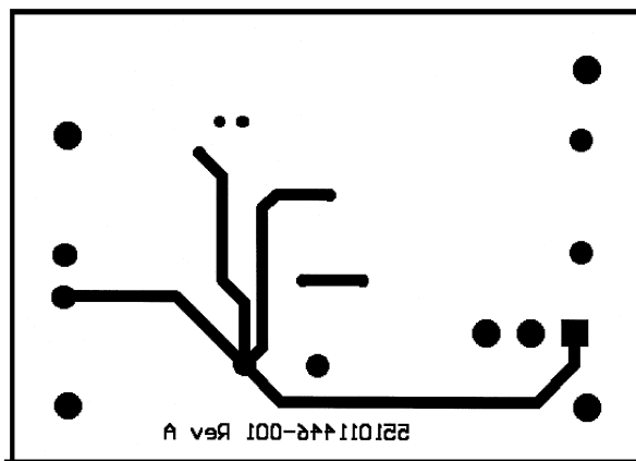
Figure 16. Bottom Layer
