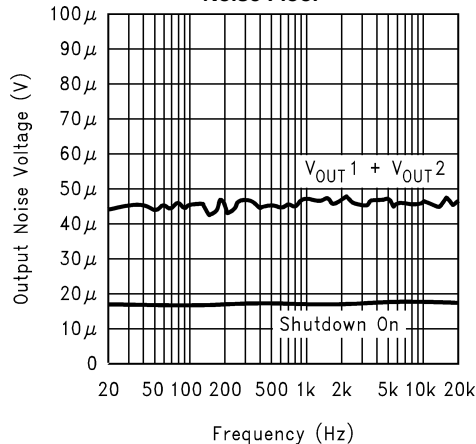
Noise Floor
