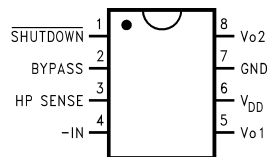
Figure 4. Mini Small Outline (MSOP) Package (Top View)
