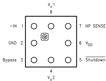
Figure 2. 8 Bump micro SMD (Top View)
