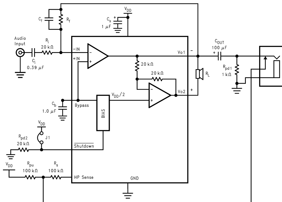
Figure 14. Higher Gain Audio Amplifier
