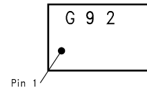
Figure 7. MSOP Marking (Top View) G - Boomer Family 92 - LM4892MM
