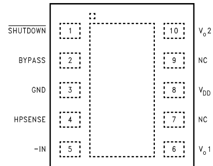
Figure 8. LLP Package (Top View)
