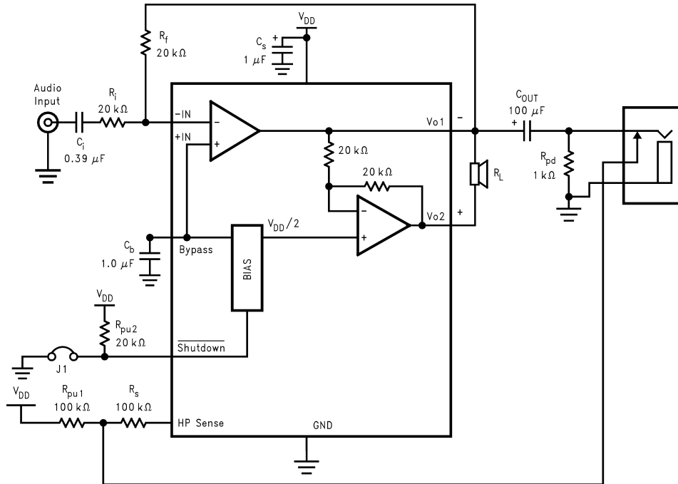
Figure 15. Reference Design Schematic For Demo Boards
