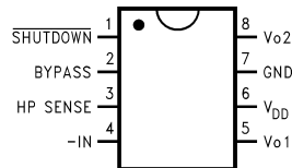
Figure 3. Small Outline (SO) Package (Top View)
