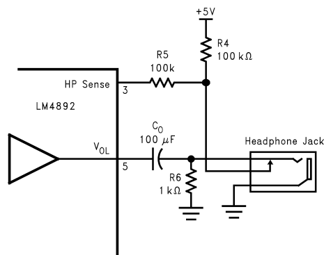
Figure 13. Headphone Circuit (Pin #'s apply to M & MM packages)
