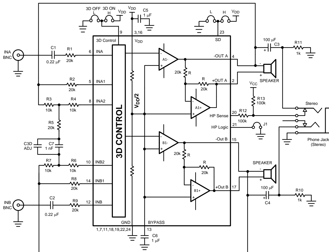
Figure 3. Typical Audio Amplifier Application Circuit
