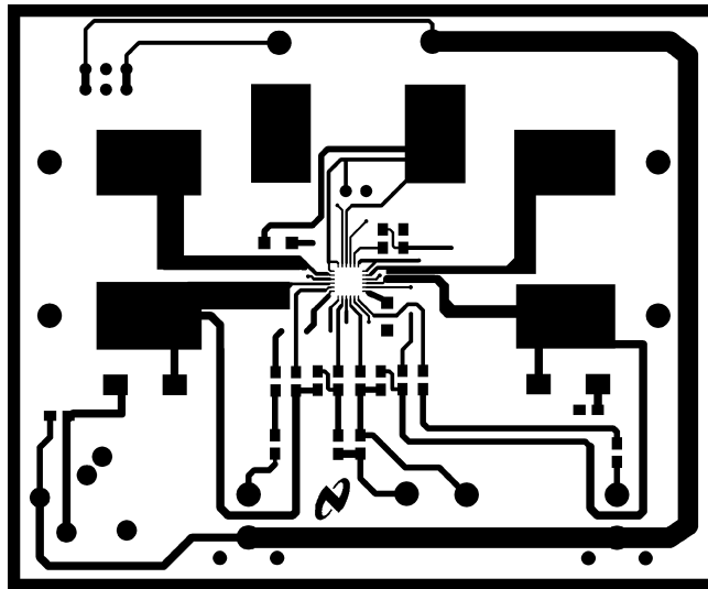
Figure 6. Top Layer
