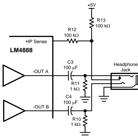
Figure 4. Headphone Circuit
