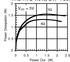
Single Channel, f = 1\text{ kHz} , THD+N \leq 1.0\% , BW < 80\text{ kHz}
