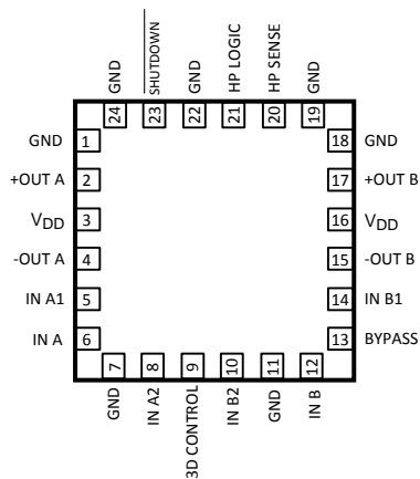
Figure 1. LM4888SQ (Top View)
