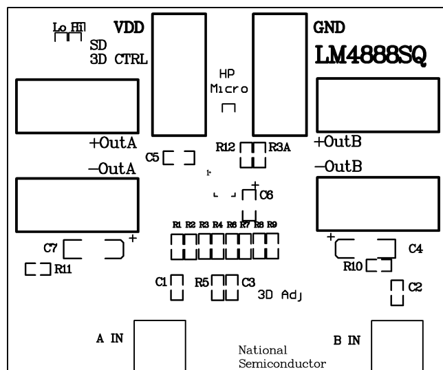
Figure 5. Silkscreen
