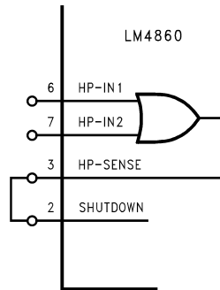
Figure 5. HP-SENSE Pin to SHUTDOWN Pin Connection
