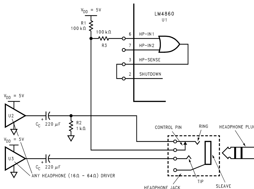
Figure 6. Typical Headphone Control Input Circuitry
