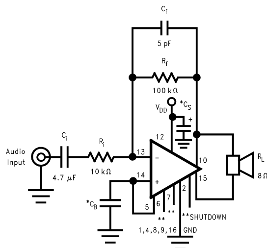
Figure 3. Stereo Amplifier with A_{vD} = 20
