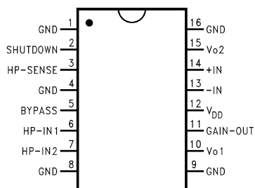
Figure 2. Small Outline Package Top View
