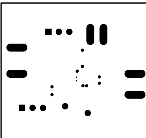
Figure 23. Bottom Silkscreen
