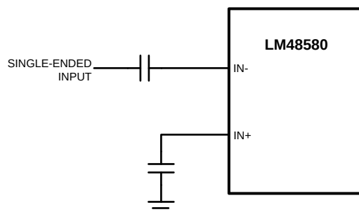
Figure 18. Single-Ended Configuration
