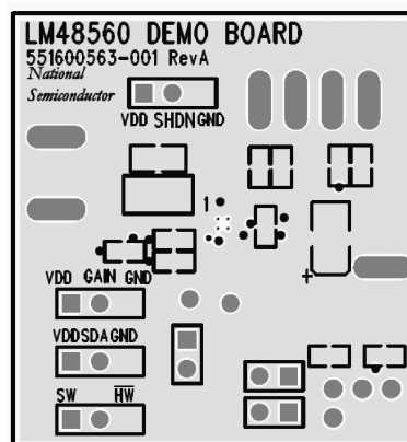
Figure 33. Layer 2
