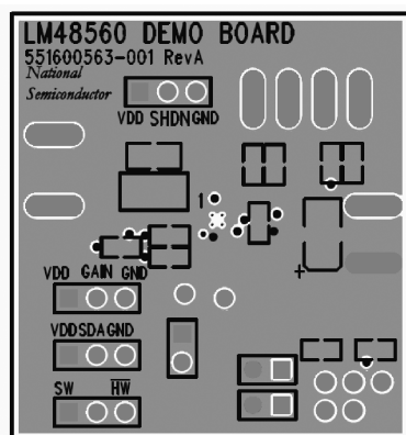
Figure 34. Layer 3
