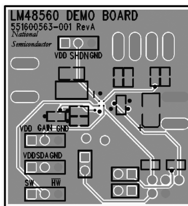
Figure 38. Bottom Layer
