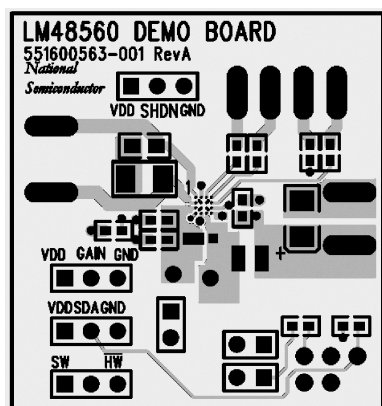
Figure 32. Top Layer
