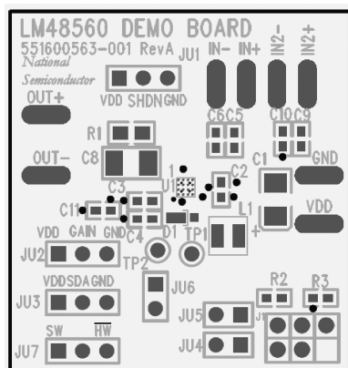
Figure 30. Top Silk Screen
