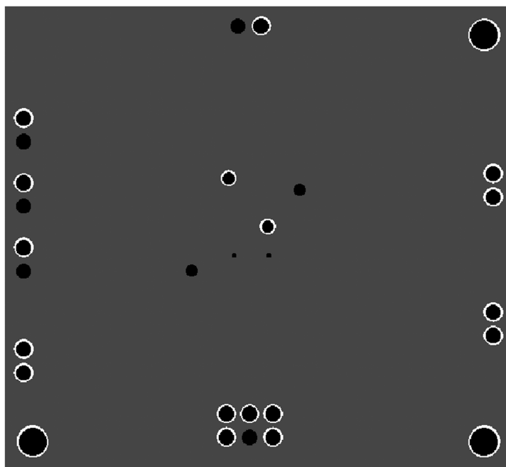
Figure 10. Recommended IBL, ITL PC Board Layout: Bottom Layer
