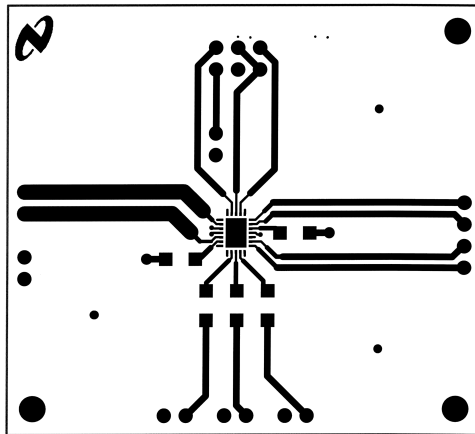
Figure 12. Recommended LQ PC Board Layout: Top Layer
