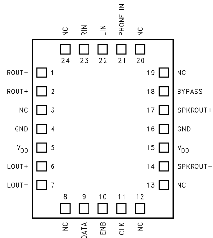
Figure 5. Top View
