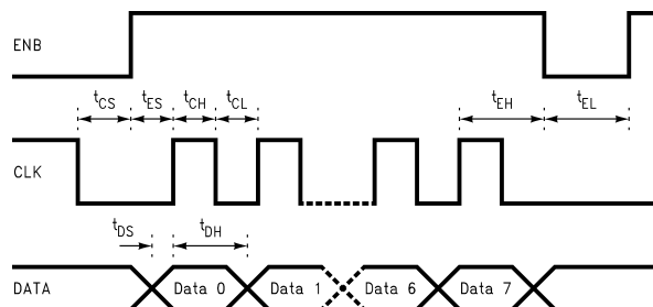
Figure 6. SPI Timing Diagram
