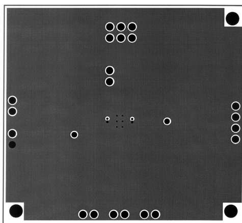
Figure 15. Recommended LQ PC Board Layout: Bottom Layer
