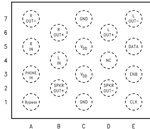
Figure 4. NC = NO CONNECT Top View (Bump-side down)
