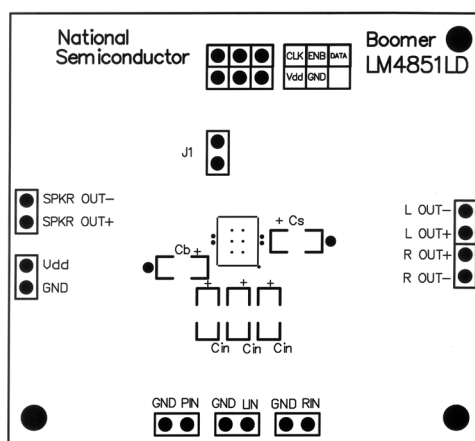
Figure 11. Recommended LQ PC Board Layout: Top Silkscreen Layer
