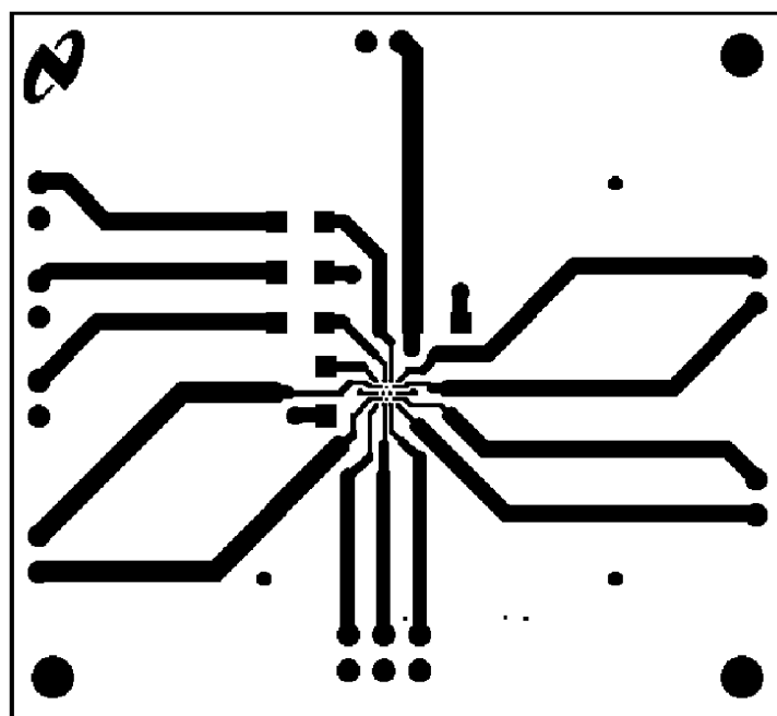
Figure 9. Recommended IBL, ITL PC Board Layout: Top Layer
