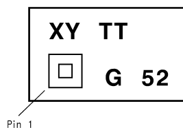
Figure 2. 18-Bump micro SMD Marking (IBL) (Top View)
