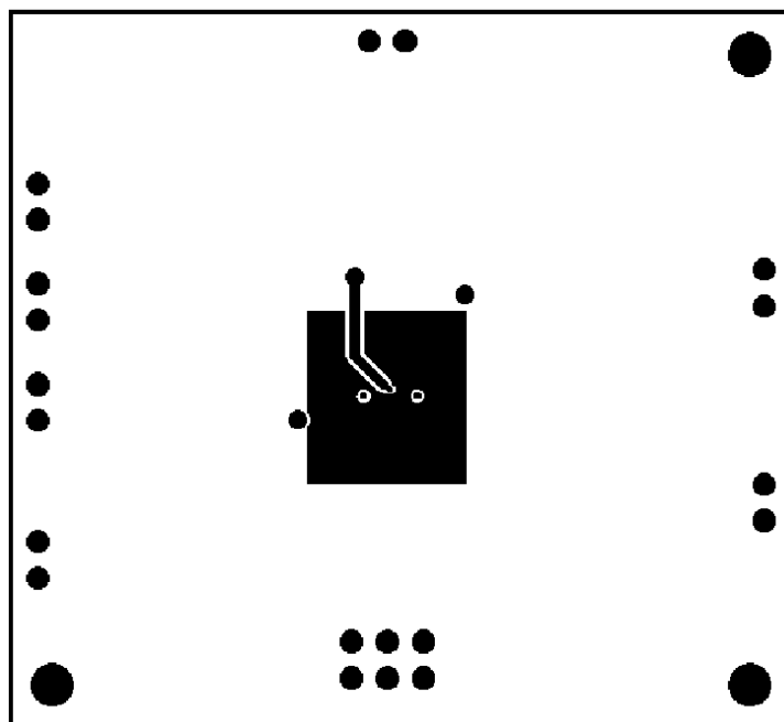
Figure 8. Recommended IBL, ITL PC Board Layout: Inner Layer
