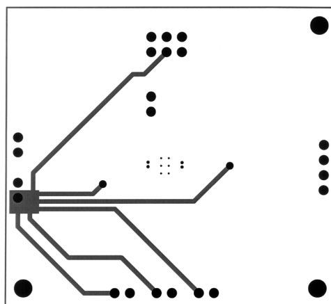
Figure 14. Recommended LQ PC Board Layout: Inner Layer 2
