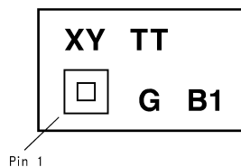
Figure 3. 18-Bump micro SMD Marking (ITL) (Top View)
