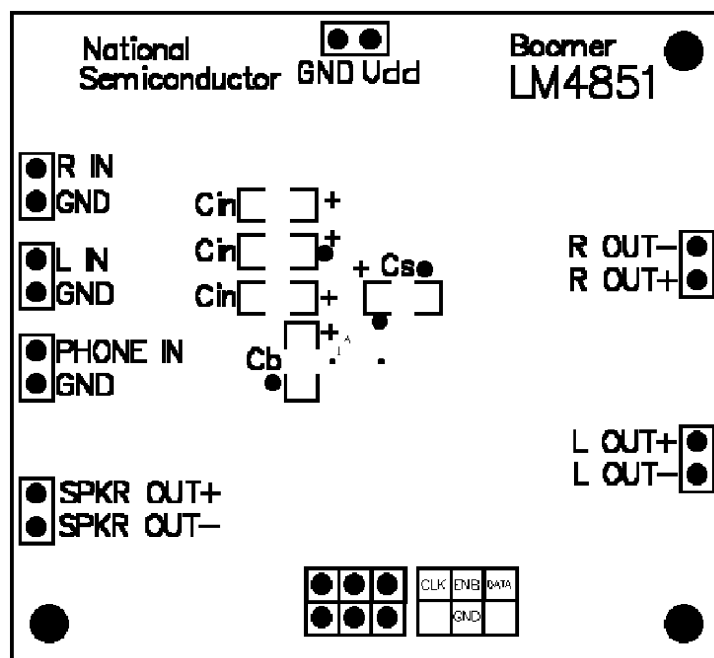
Figure 7. Recommended IBL, ITL PC Board Layout: Top Silkscreen
