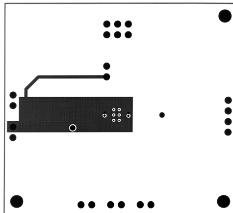
Figure 13. Recommended LQ PC Board Layout: Inner Layer 1
