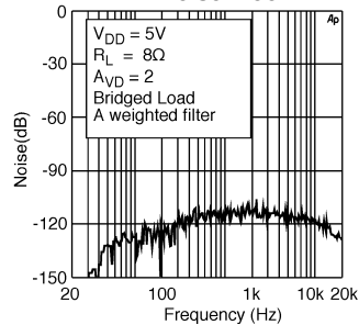
Noise Floor
