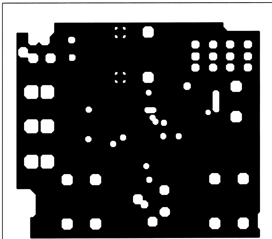
Figure 11. Recommended LQ PC Board Layout: Lower Inner-Layer Layout
