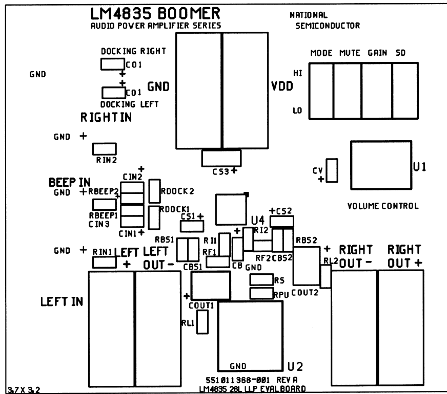
Figure 8. Recommended LQ PC Board Layout: Component-Side Silkscreen
