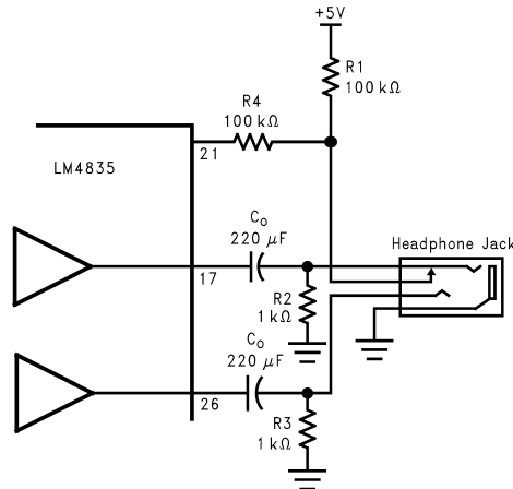
Figure 6. Headphone Sensing Circuit
