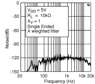
Noise Floor
