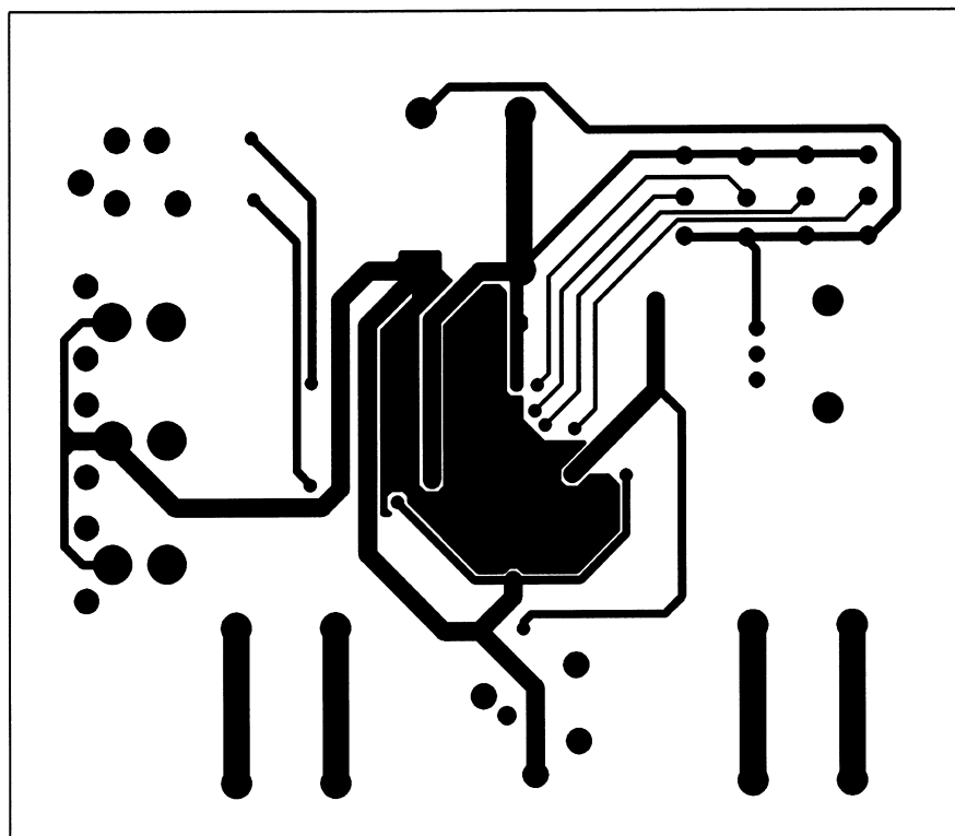
Figure 12. Recommended LQ PC Board Layout: Bottom-Side Layout
