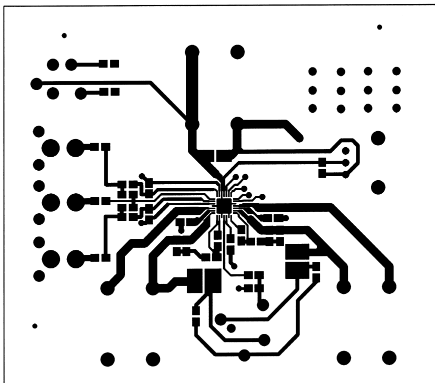
Figure 9. Recommended LQ PC Board Layout: Component-Side Layout
