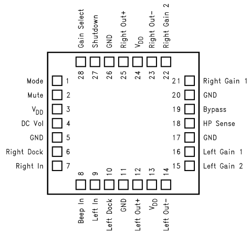
Figure 1. LLP Package - Top View
