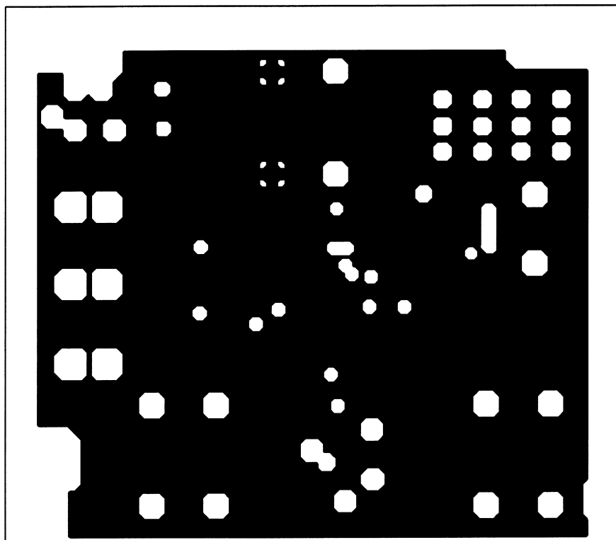
Figure 10. Recommended LQ PC Board Layout: Upper Inner-Layer Layout
