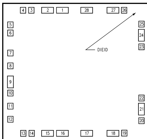
Figure 13. Die Layout (A - Step)
