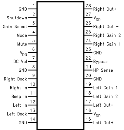
Figure 2. TSSOP Package - Top View
