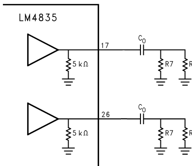
Figure 5. Resistor for Varying Output Loads
