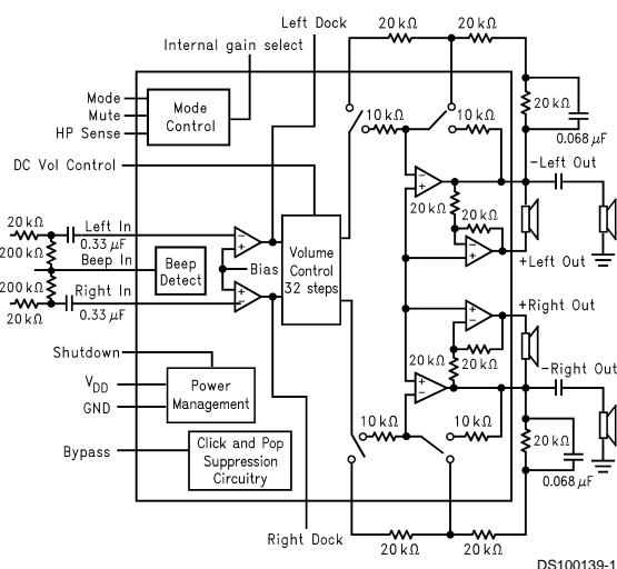
FIGURE 1. LM4835 Block Diagram
