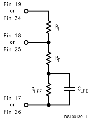
FIGURE 5. Low Frequency Enhancement
