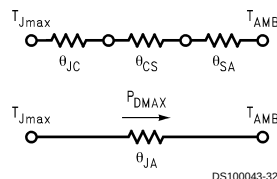
FIGURE 8. Thermal Model
