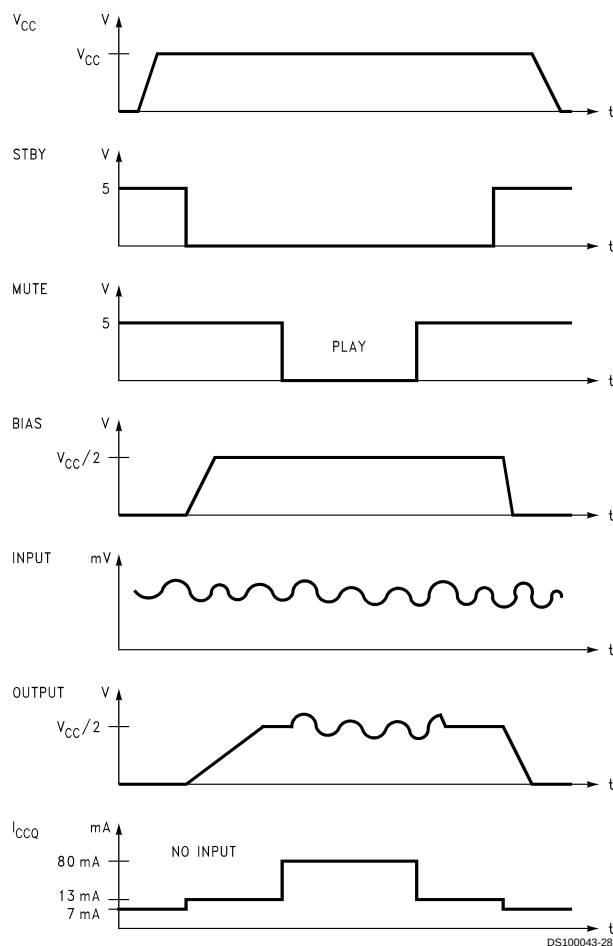
FIGURE 4. Turn-On/Off Sequence
