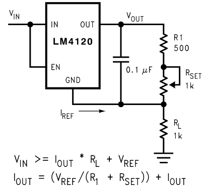
Figure 30. Programmable Current Source
