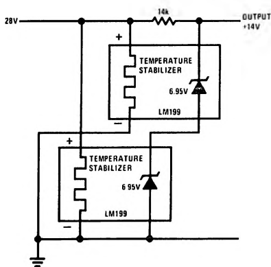
14V Reference
