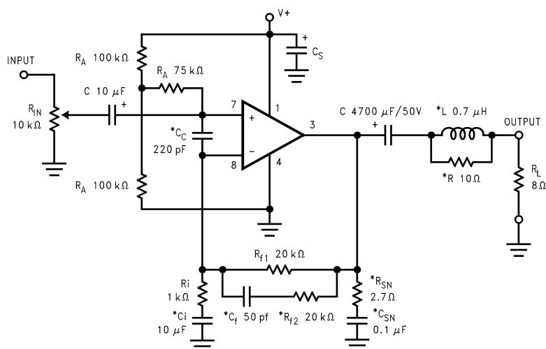
Figure 3. Typical Single Supply Audio Amplifier Application Circuit
