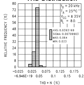
THD Distribution
