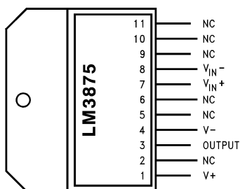
Figure 2. Plastic Package (1) Top View
