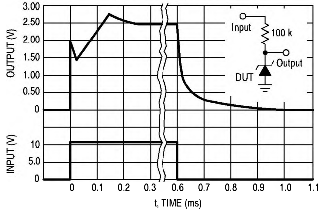
Figure 12. Response Time
