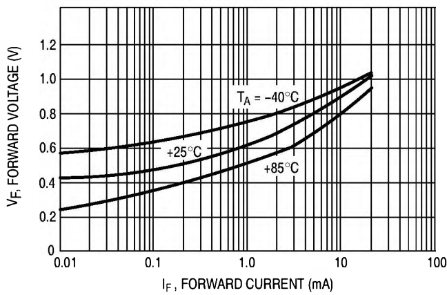
Figure 3. Forward Characteristics
