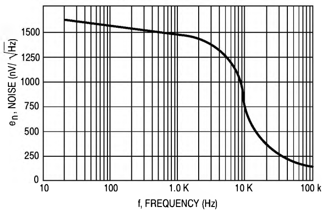
Figure 11. Noise Voltage
