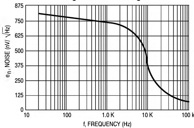
Figure 5. Noise Voltage
