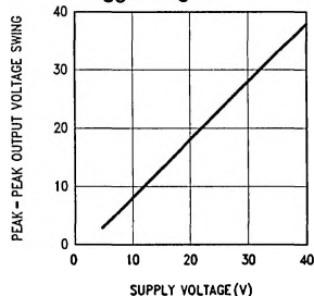
P-P Output Voltage V_{CC} Swing vs
