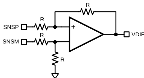
Figure 18. Differential Amplifier
