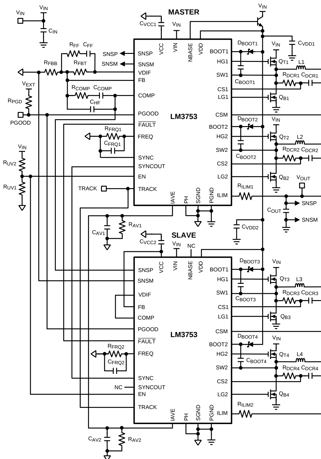
Figure 31. Typical Application
