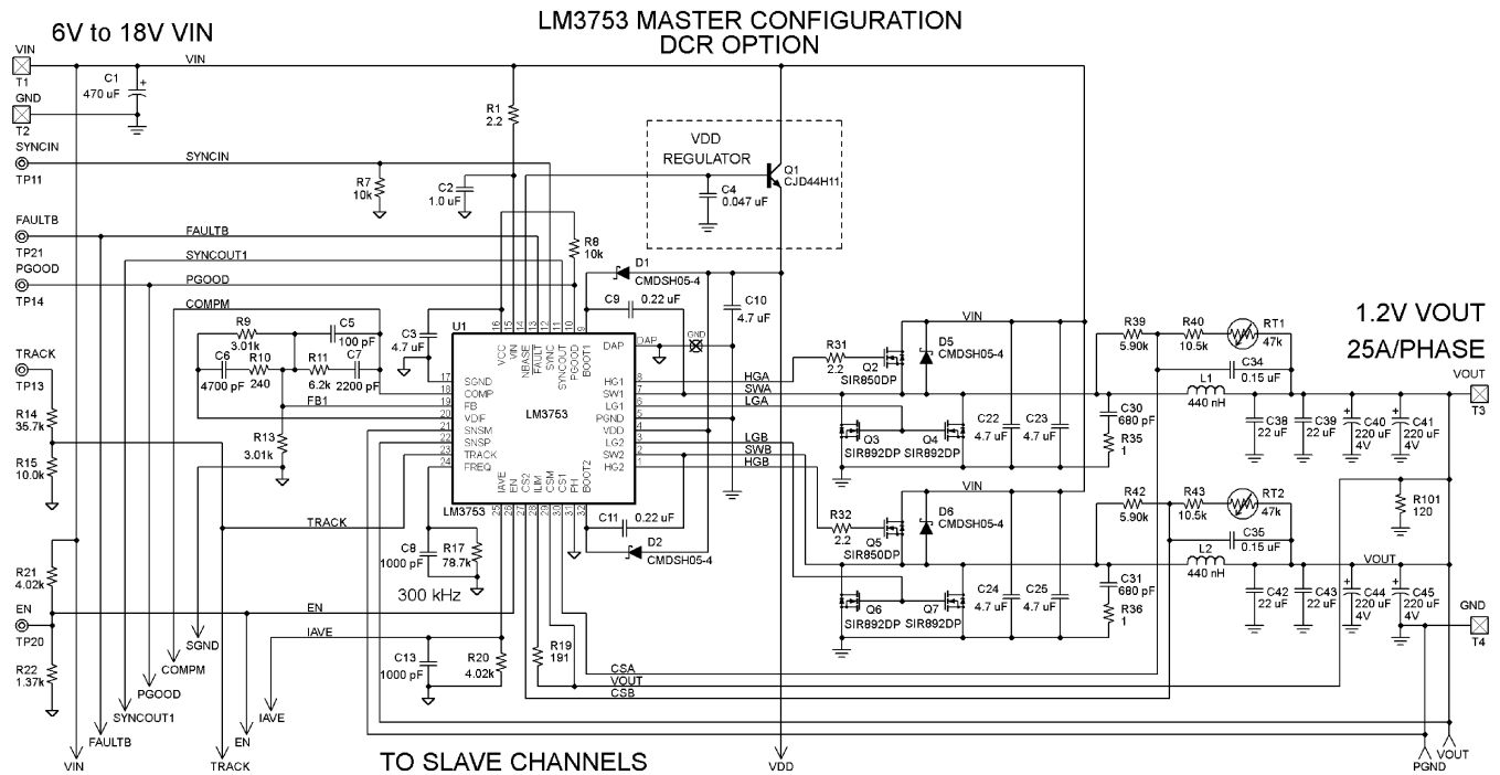
Figure 32. Master with DCR Sense
