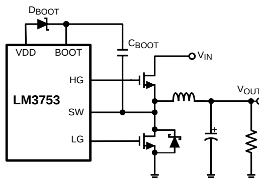
Figure 17. Bootstrap Circuit
