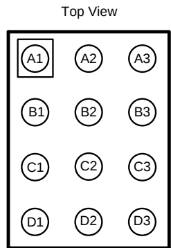
Figure 3. DSBGA Package see package number YFQ0012AAA
