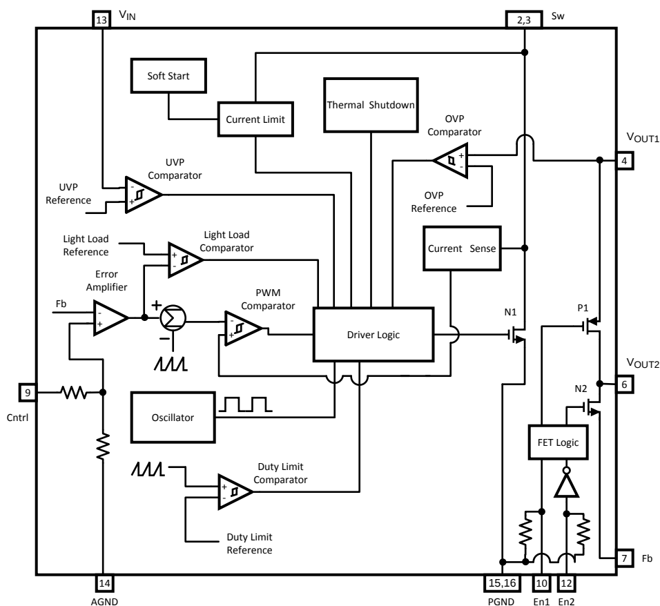
Figure 3. Block Diagram
