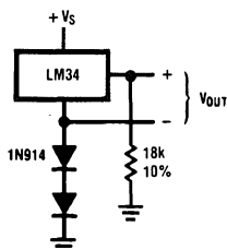
Temperature Sensor, Single Supply, -50^{\circ} to +300^{\circ}\text{F}
