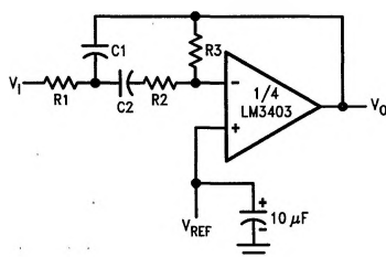
Multiple Feedback Bandpass Filter
