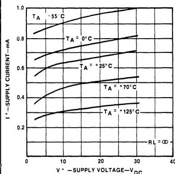
SUPPLY CURRENT
