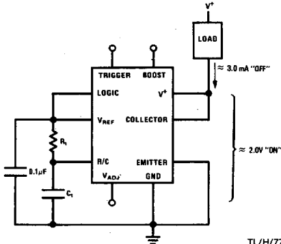
FIGURE 9. 2-Terminal Time Delay Switch
