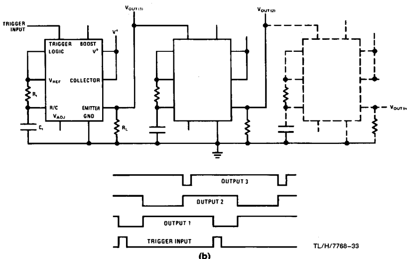
FIGURE 20. Chain of Timers
