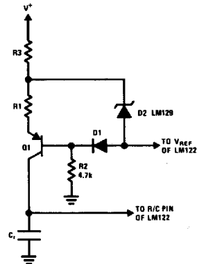
FIGURE 18. Temperature Compensated Linear Charging Sweep
