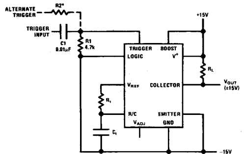
FIGURE 17. Operating Off Dual Supplies
