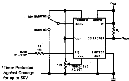
FIGURE 15. Comparator with 0V to 3V Threshold
