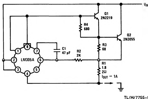
Current Regulator
