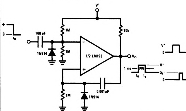
One-Shot Multivibrator
