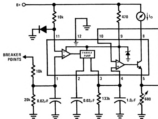
Current Driven Meter Indicating Engine RPM I_0 = 10 \text{ mA @ 300 Hz or 6000 ERPM (6 Cylinder Engine)}
