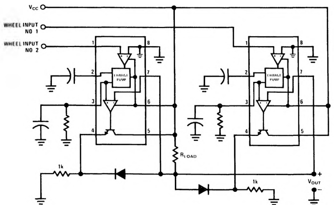
“Select-Low” Circuit
