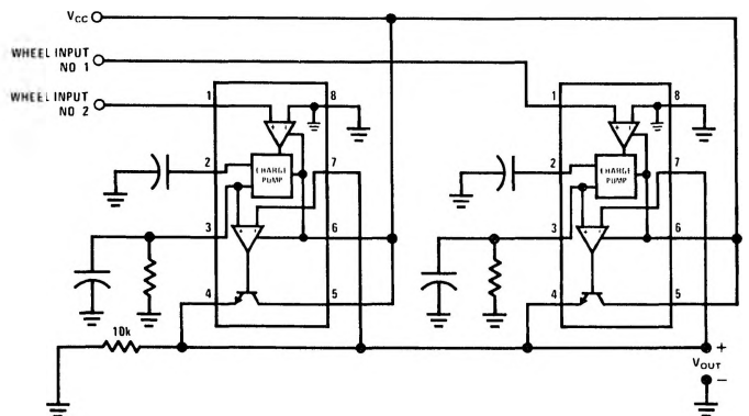
“Select-High” Circuit
