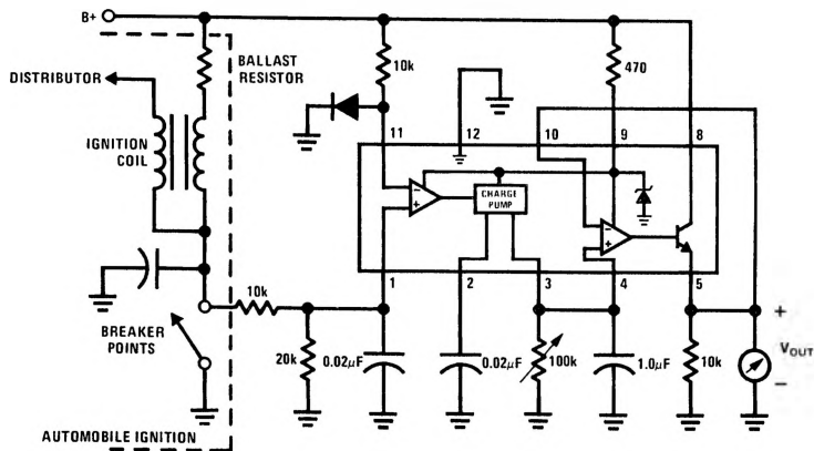
Voltage Driven Meter Indicating Engine RPM V_O = 6V @ 400 \text{ Hz} or 6000 ERPM (8 Cylinder Engine)
