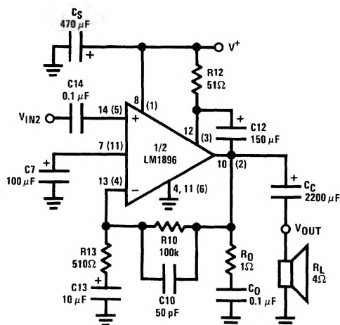
FIGURE 2. Stereo Amplifier with A_V = 200 , BW = 30 kHz
