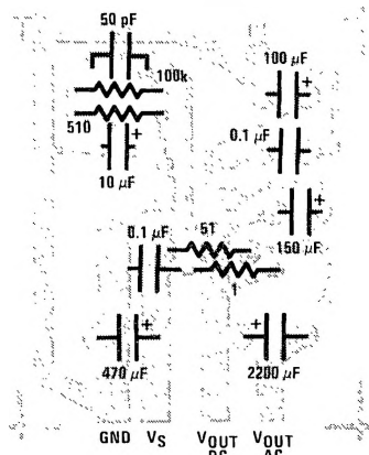
FIGURE 4. Printed Circuit Board Layout for LM1895
