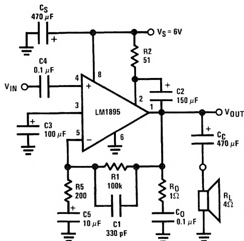
FIGURE 1. LM1895 with A_V = 500 , BW = 5 kHz, AM Radio Application ( V_{IN} = 4.2\text{ mV} for Full Power Output)
