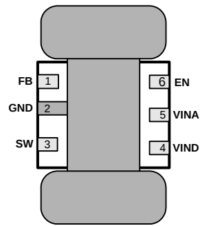
Figure 6. 6-Lead LLP PCB Dog Bone Layout
