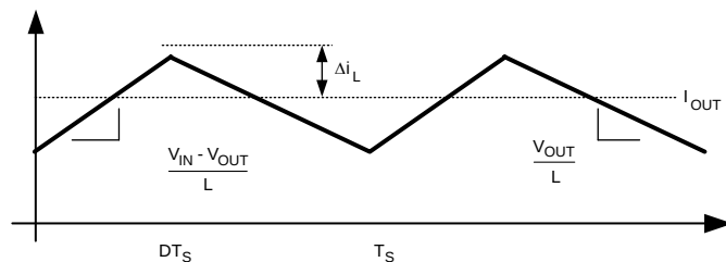
Figure 4. Inductor Current
