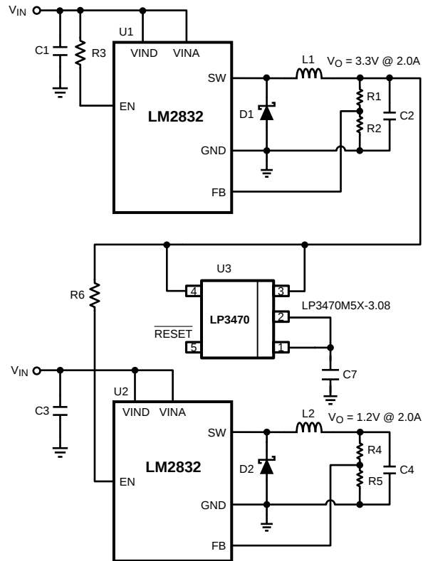
Figure 14. LM2832X (1.6MHz): Vin = 5V, Vo = 1.2V @ 2.0A & 3.3V @2.0A
