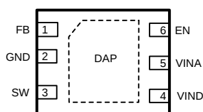
Figure 1. 6-Pin LLP
