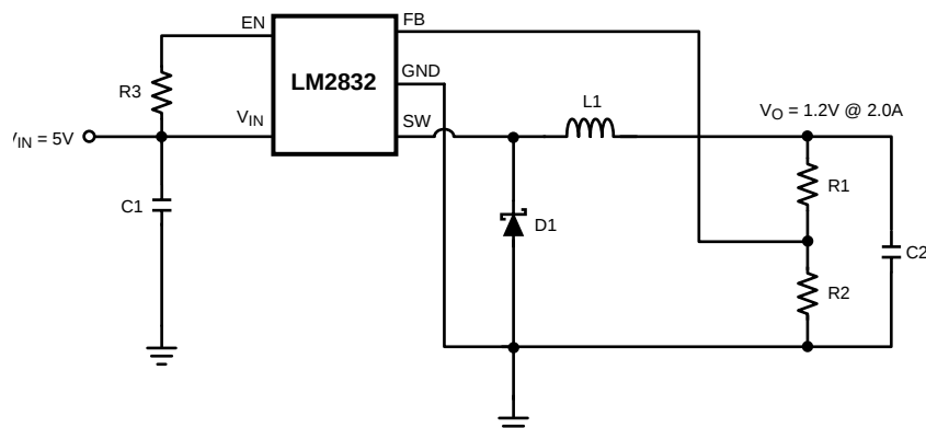
Figure 13. LM2832Z (3MHz): V_{IN} = 5V , V_O = 1.2V @ 2.0A
