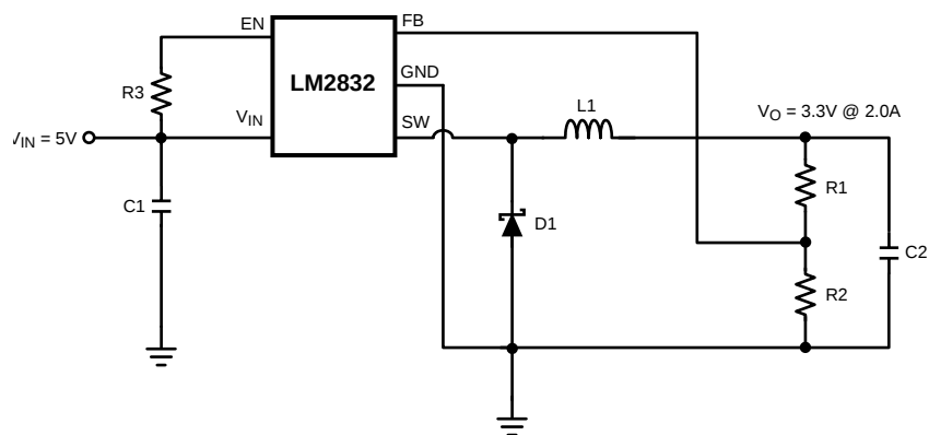
Figure 12. LM2832Z (3MHz): V in = 5V, V o = 3.3V @ 2.0A
