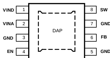
Figure 2. 8-Pin eMSOP
