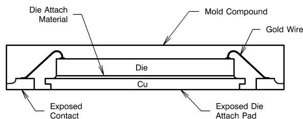
Figure 5. Internal LLP Connection
