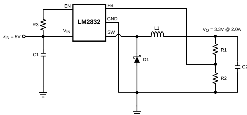
Figure 10. LM2832Y (550kHz): V_{in} = 5V , V_{out} = 3.3V @ 2.0A
