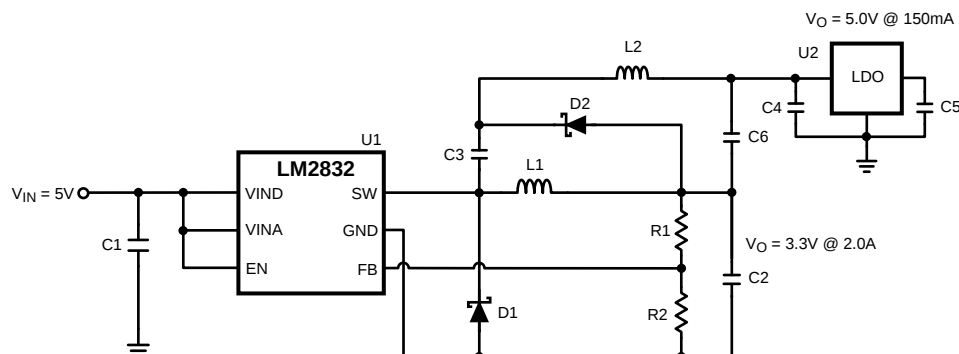
Figure 15. LM2832X (1.6MHz): V_{in} = 5V , V_o = 3.3V @ 2.0A & LP2986-5.0 @ 150mA
