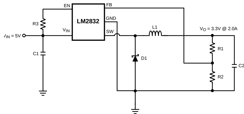
Figure 9. LM2832X (1.6MHz): V_{IN} = 5V , V_O = 3.3V @ 2.0A
