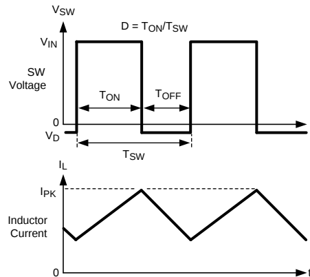
Figure 3. Typical Waveforms
