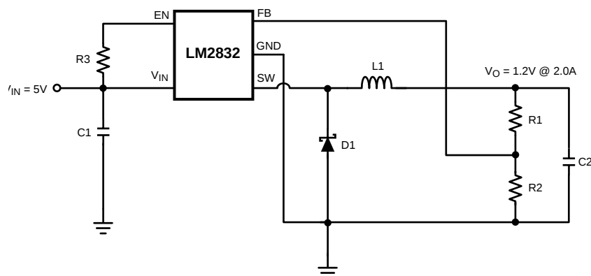
Figure 11. LM2832Y (550kHz): V_{in} = 5V , V_{out} = 1.2V @ 2.0A
