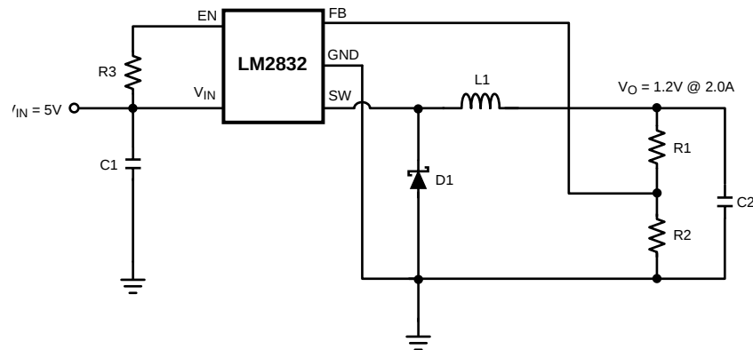
Figure 7. LM2832X (1.6MHz): V_{in} = 5V , V_o = 1.2V @ 2.0A
