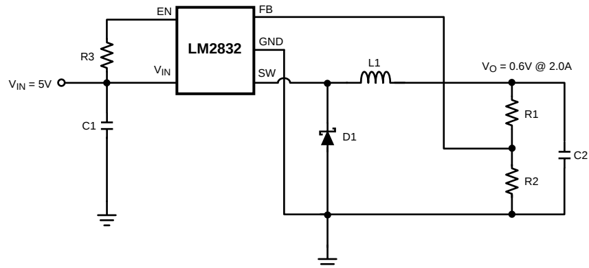
Figure 8. LM2832X (1.6MHz): V_{IN} = 5V , V_O = 0.6V @ 2.0A
