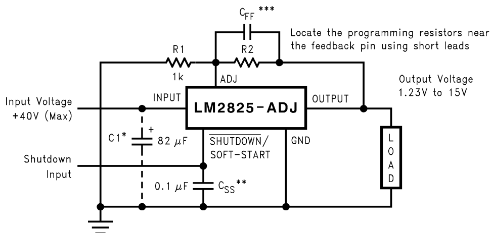
Figure 17. Standard Test Circuit (Fixed Output Voltage Versions)
