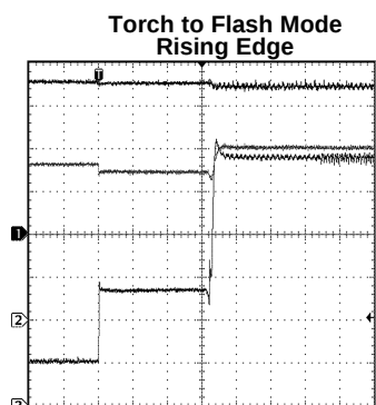
V_{IN} = 3.6\text{V} , Load = 200mA/800mA (Torch/Flash), LED = PWF1 CH1 (TOP): V_{IN} ; Scale: 1V/Div, DC Coupled CH2 (MIDDLE): V_{OUT} ; Scale: 1V/Div, DC Coupled CH3 (BOTTOM): I_{IN} ; Scale: 200mA/Div Time scale: 400μs/Div
