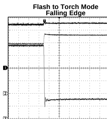
V_{IN} = 3.6\text{V} , Load = 800mA/200mA (Flash/Torch), LED = PWF1 CH1 (TOP): V_{IN} ; Scale: 1V/Div, DC Coupled CH2 (MIDDLE): V_{OUT} ; Scale: 1V/Div, DC Coupled CH3 (BOTTOM): I_{IN} ; Scale: 200mA/Div Time scale: 100μs/Div
